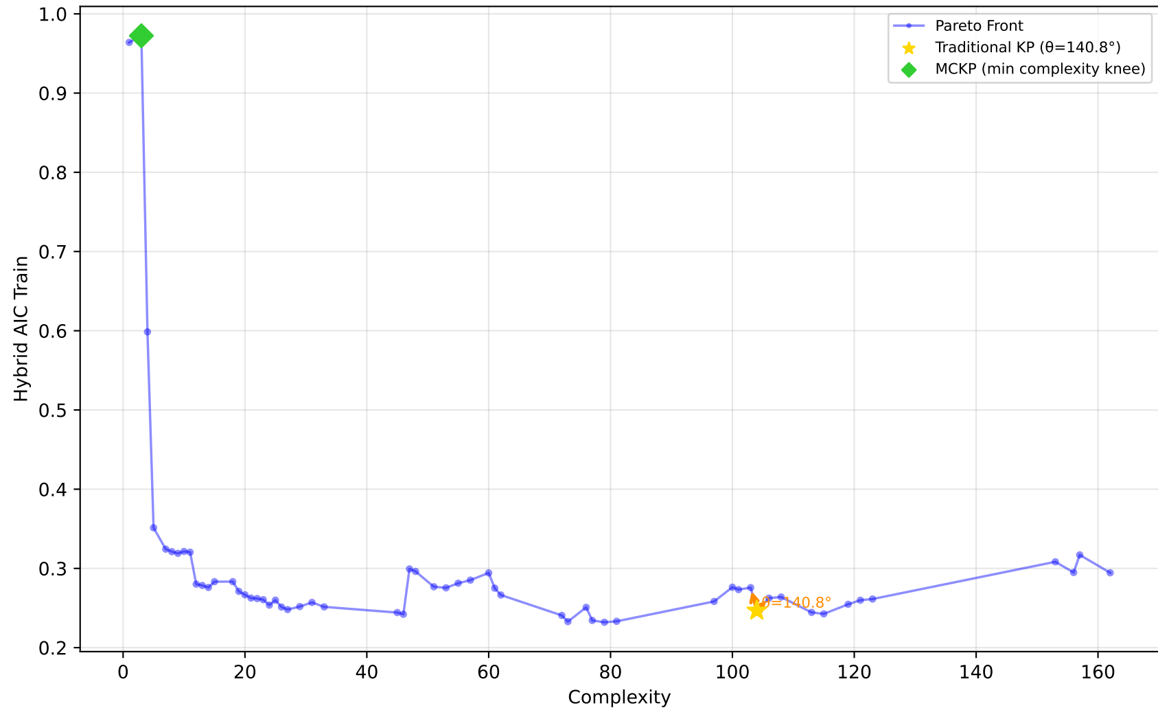
712_chscase_geyser1 - Run 7 - SVP - Hybrid AIC Train \lambda_1=1.00, \lambda_2=1.00, \lambda_3=0.00 | Difficulty: 1.00 | Method: hmr
