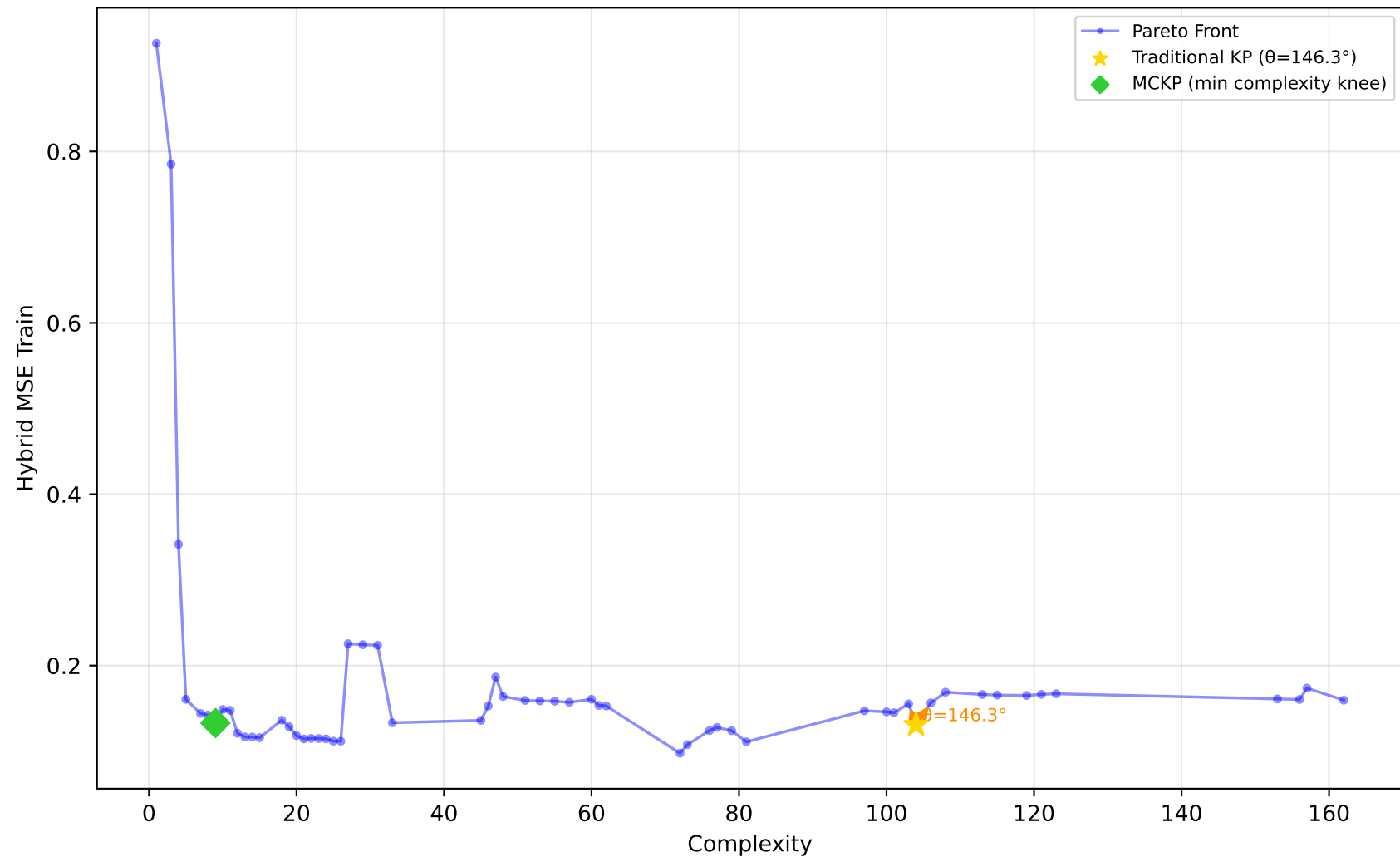
712_chscase_geyser1 - Run 7 - SVP - Hybrid MSE Train \lambda_1=0.00, \lambda_2=1.00, \lambda_3=1.00 | Difficulty: 1.00 | Method: hmr
