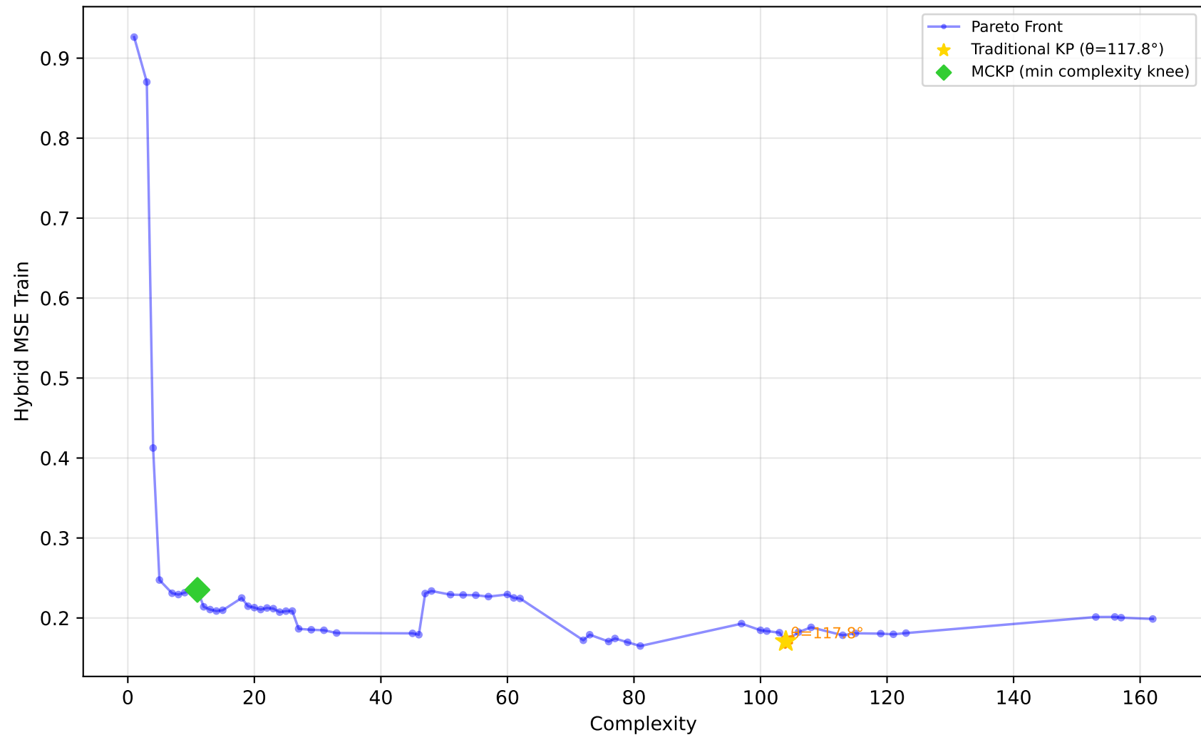
712_chscase_geyser1 - Run 7 - SVP - Hybrid MSE Train \lambda_1=1.00, \lambda_2=1.00, \lambda_3=0.00 | Difficulty: 1.00 | Method: hmr
