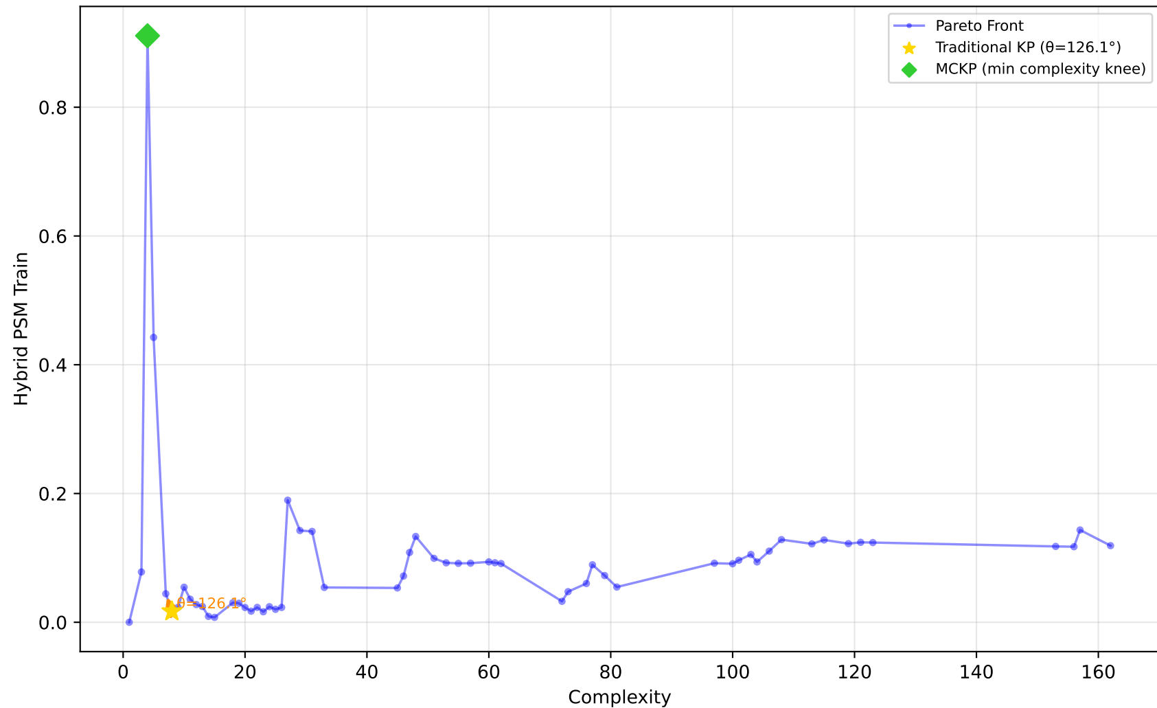
712_chscase_geyser1 - Run 7 - SVP - Hybrid PSM Train \lambda_1=0.00, \lambda_2=1.00, \lambda_3=1.00 | Difficulty: 1.00 | Method: hmr
