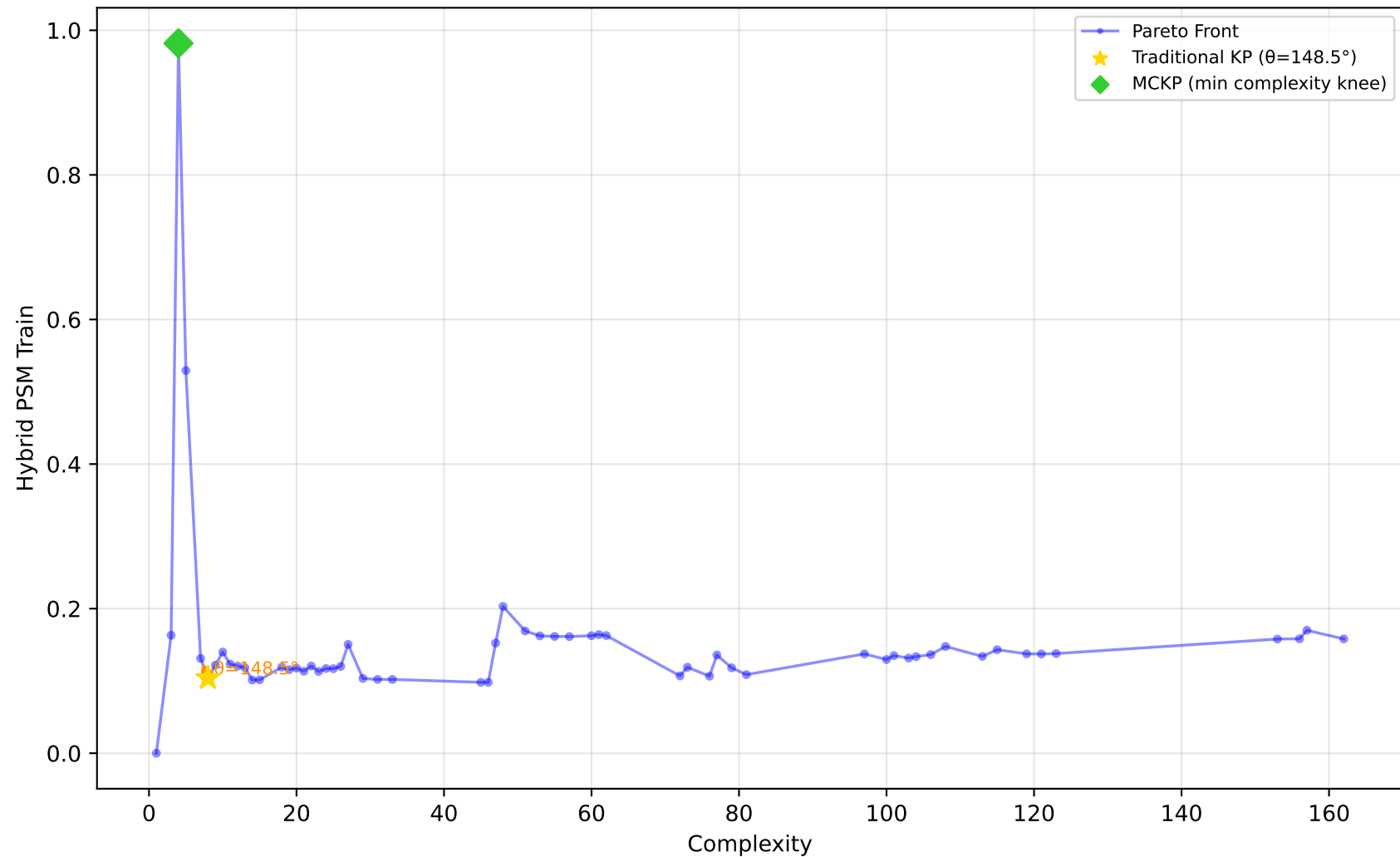
712_chscase_geyser1 - Run 7 - SVP - Hybrid PSM Train \lambda_1=1.00, \lambda_2=1.00, \lambda_3=0.00 | Difficulty: 1.00 | Method: hmr
