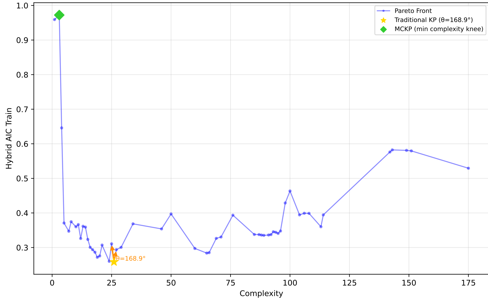
712_chscase_geyser1 - Run 8 - MVP - Hybrid AIC Train \lambda_1=1.00, \lambda_2=1.00, \lambda_3=1.00 | Difficulty: 0.66 | Method: hmr
