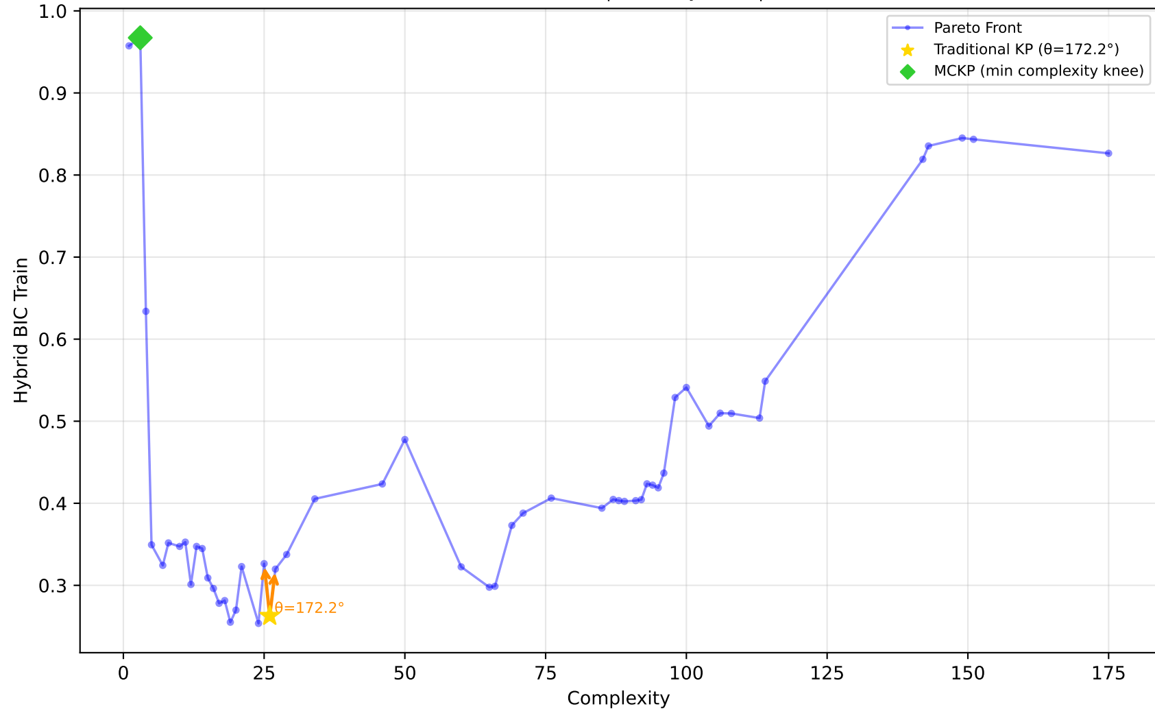
712_chscase_geyser1 - Run 8 - MVP - Hybrid BIC Train \lambda_1=1.00, \lambda_2=1.00, \lambda_3=1.00 | Difficulty: 0.66 | Method: hmr
