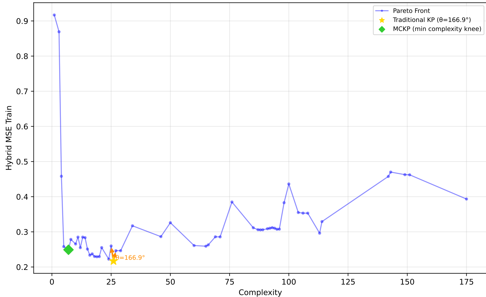
712_chscase_geyser1 - Run 8 - MVP - Hybrid MSE Train \lambda_1=1.00, \lambda_2=1.00, \lambda_3=1.00 | Difficulty: 0.66 | Method: hmr
