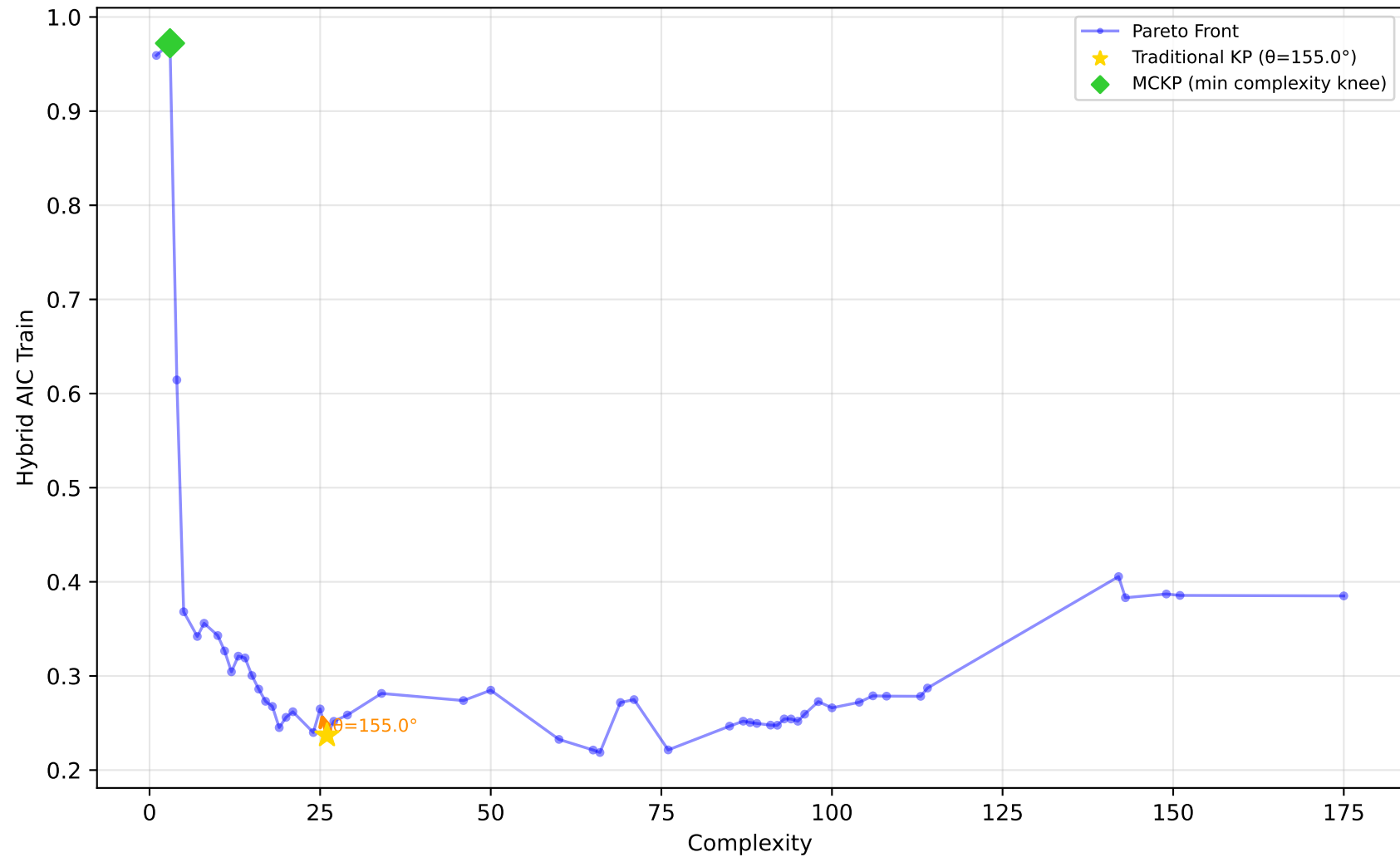
712_chscase_geyser1 - Run 8 - SVP - Hybrid AIC Train \lambda_1=1.00, \lambda_2=1.00, \lambda_3=0.00 | Difficulty: 0.66 | Method: hmr
