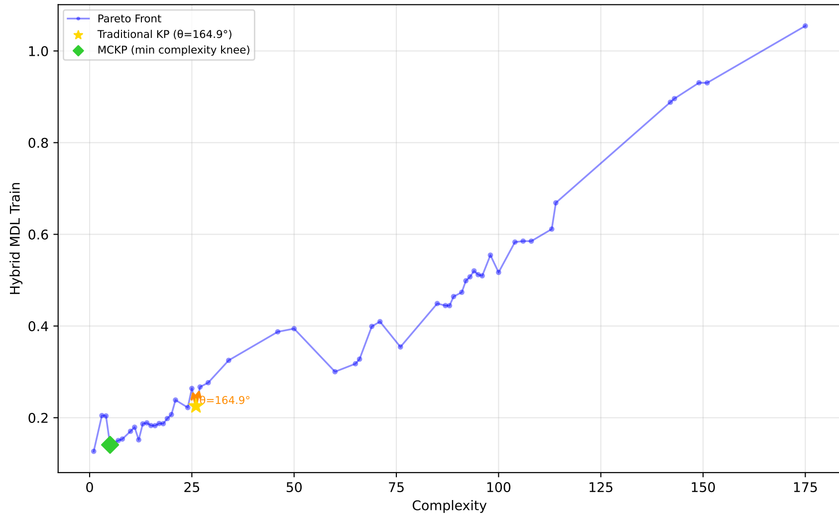
712_chscase_geyser1 - Run 8 - SVP - Hybrid MDL Train \lambda_1=1.00, \lambda_2=1.00, \lambda_3=0.00 | Difficulty: 0.66 | Method: hmr
