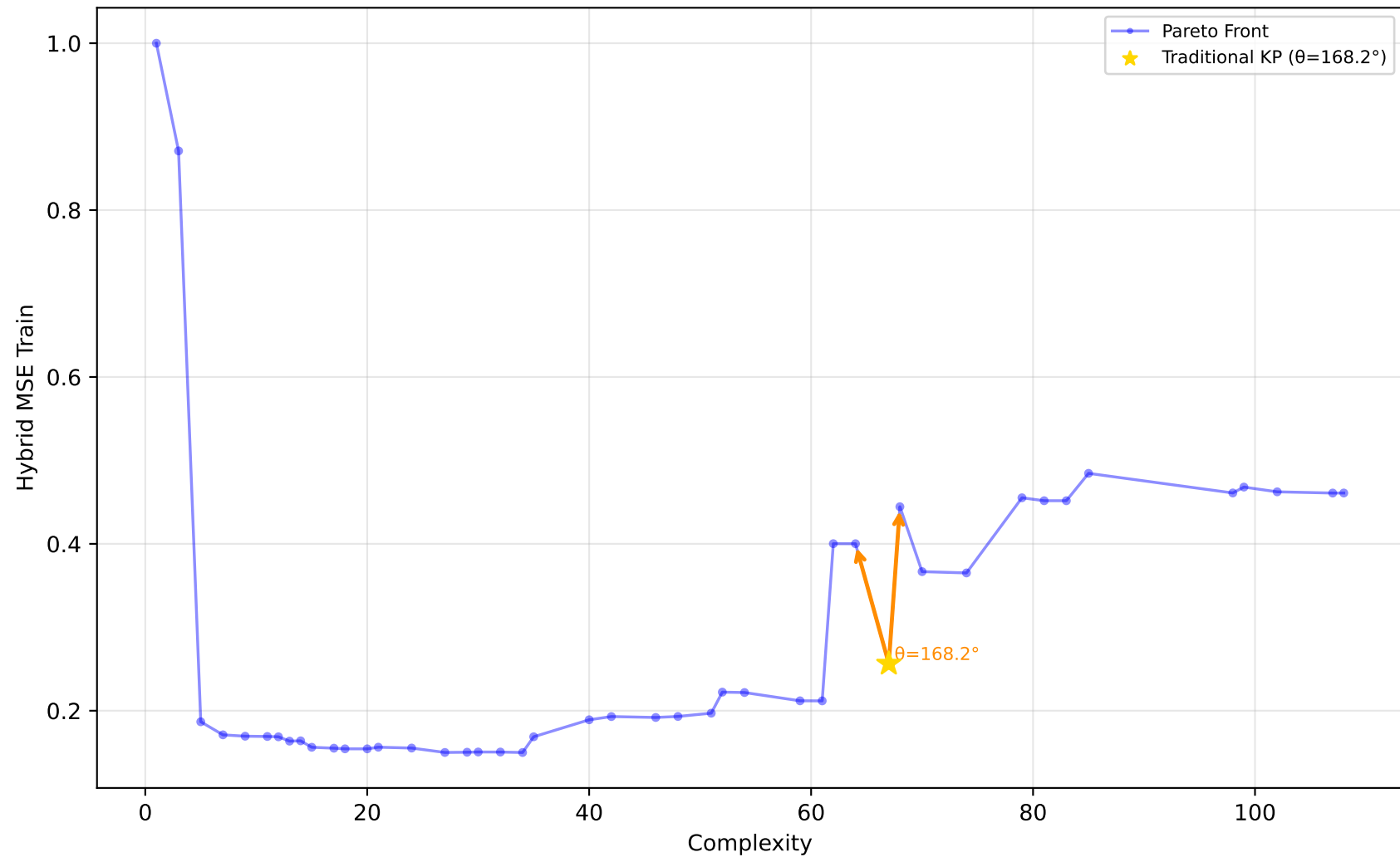
712_chscase_geyser1 - Run 9 - MVP - Hybrid MSE Train \lambda_1=0.20, \lambda_2=1.00, \lambda_3=1.00 | Difficulty: 1.00 | Method: hmr
