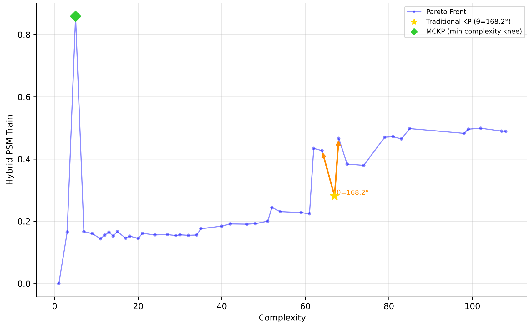
712_chscase_geyser1 - Run 9 - MVP - Hybrid PSM Train \lambda_1=1.00, \lambda_2=1.00, \lambda_3=1.00 | Difficulty: 1.00 | Method: hmr
