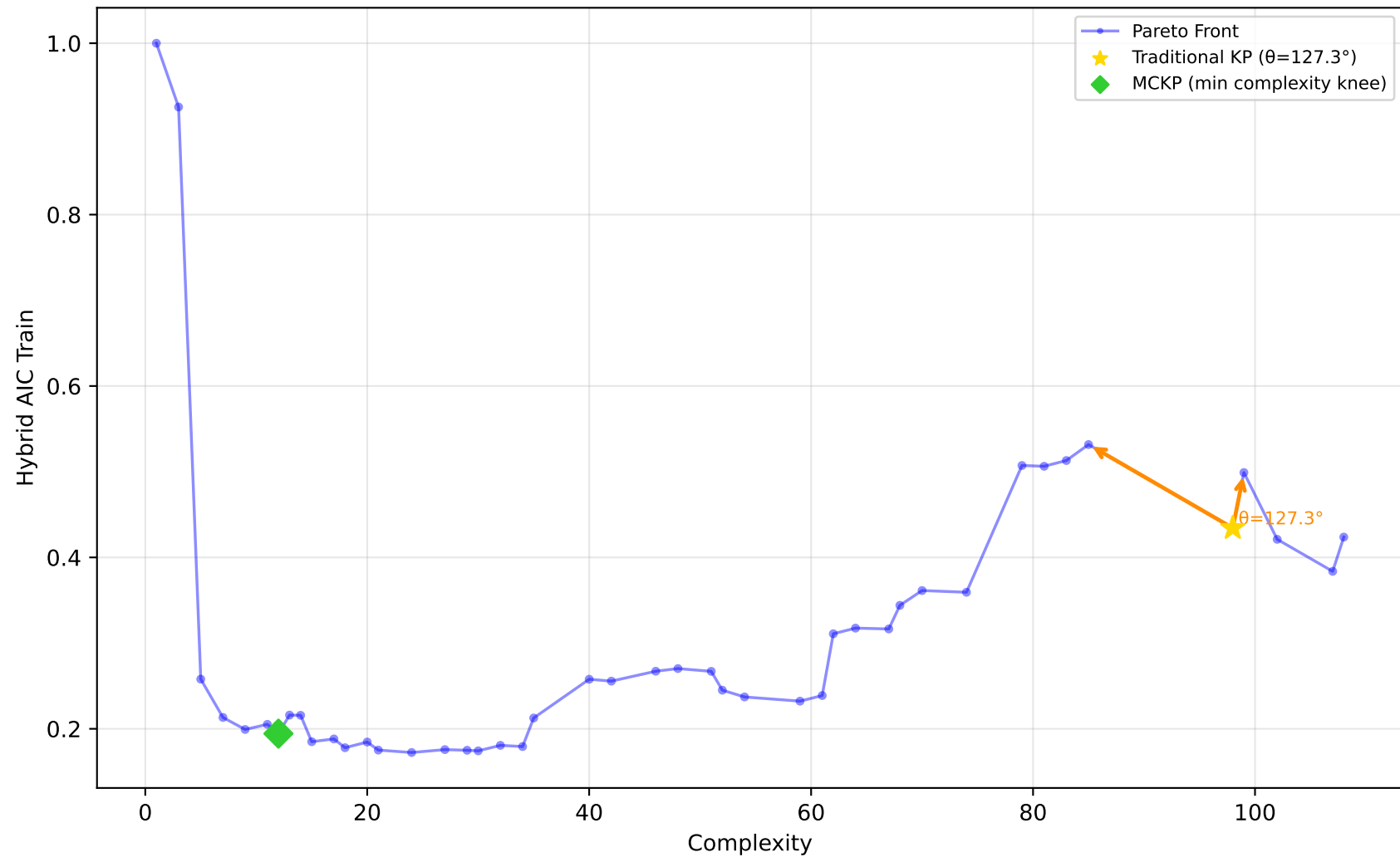
712_chscase_geyser1 - Run 9 - SVP - Hybrid AIC Train \lambda_1=0.00, \lambda_2=1.00, \lambda_3=1.00 | Difficulty: 1.00 | Method: hmr
