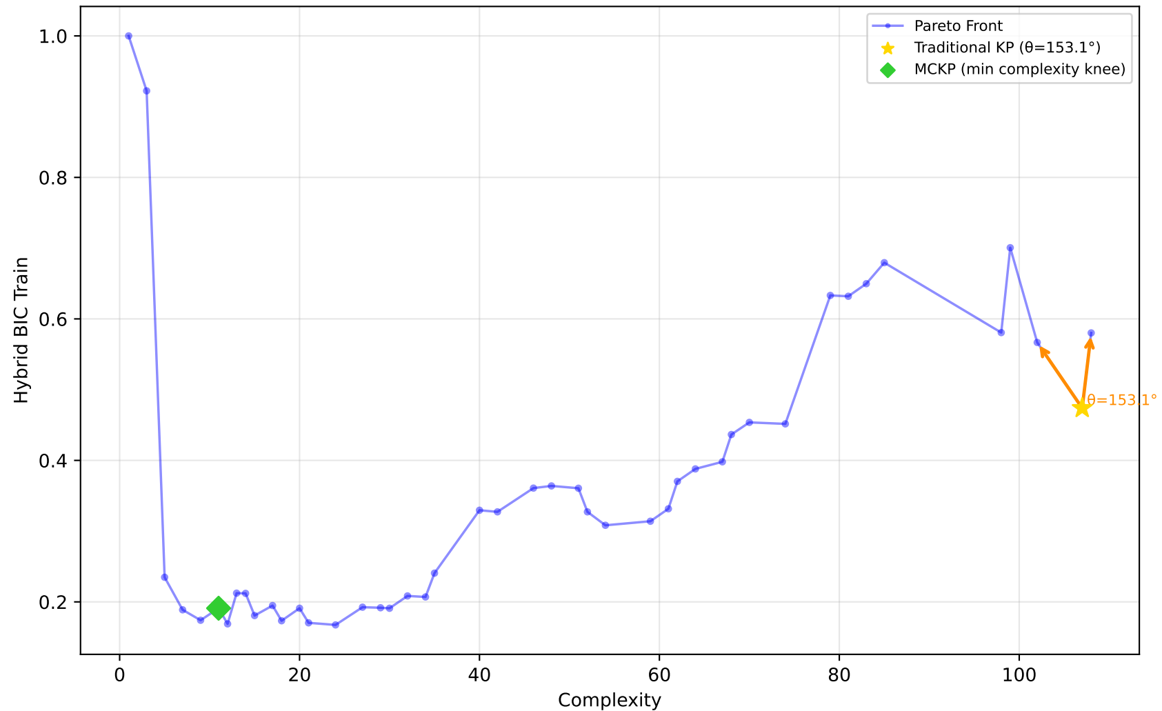
712_chscase_geyser1 - Run 9 - SVP - Hybrid BIC Train \lambda_1=0.00, \lambda_2=1.00, \lambda_3=1.00 | Difficulty: 1.00 | Method: hmr
