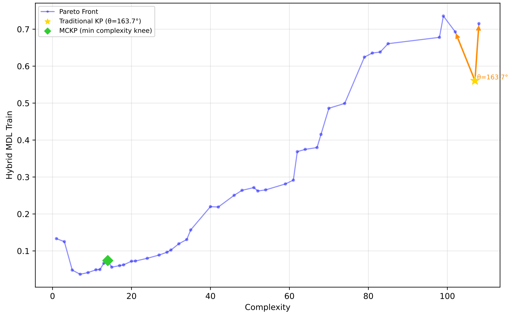
712_chscase_geyser1 - Run 9 - SVP - Hybrid MDL Train \lambda_1=0.00 , \lambda_2=1.00 , \lambda_3=1.00 | Difficulty: 1.00 | Method: hmr
