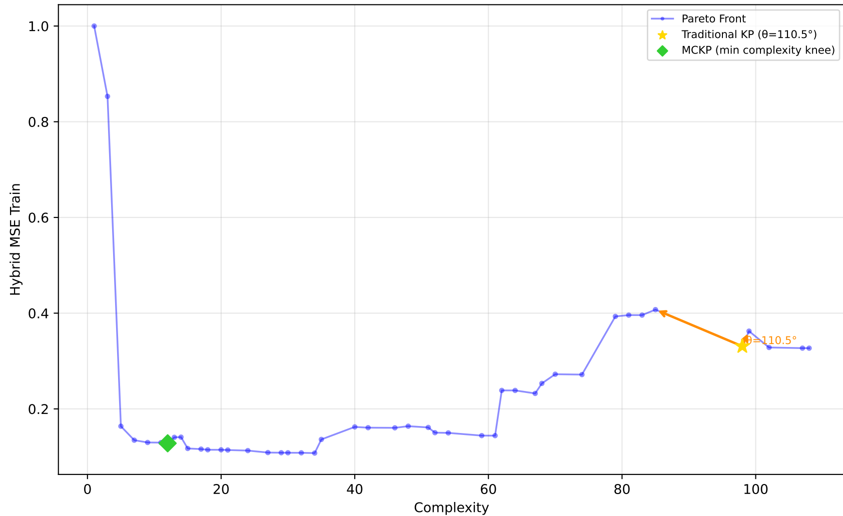
712_chscase_geyser1 - Run 9 - SVP - Hybrid MSE Train \lambda_1=0.00, \lambda_2=1.00, \lambda_3=1.00 | Difficulty: 1.00 | Method: hmr
