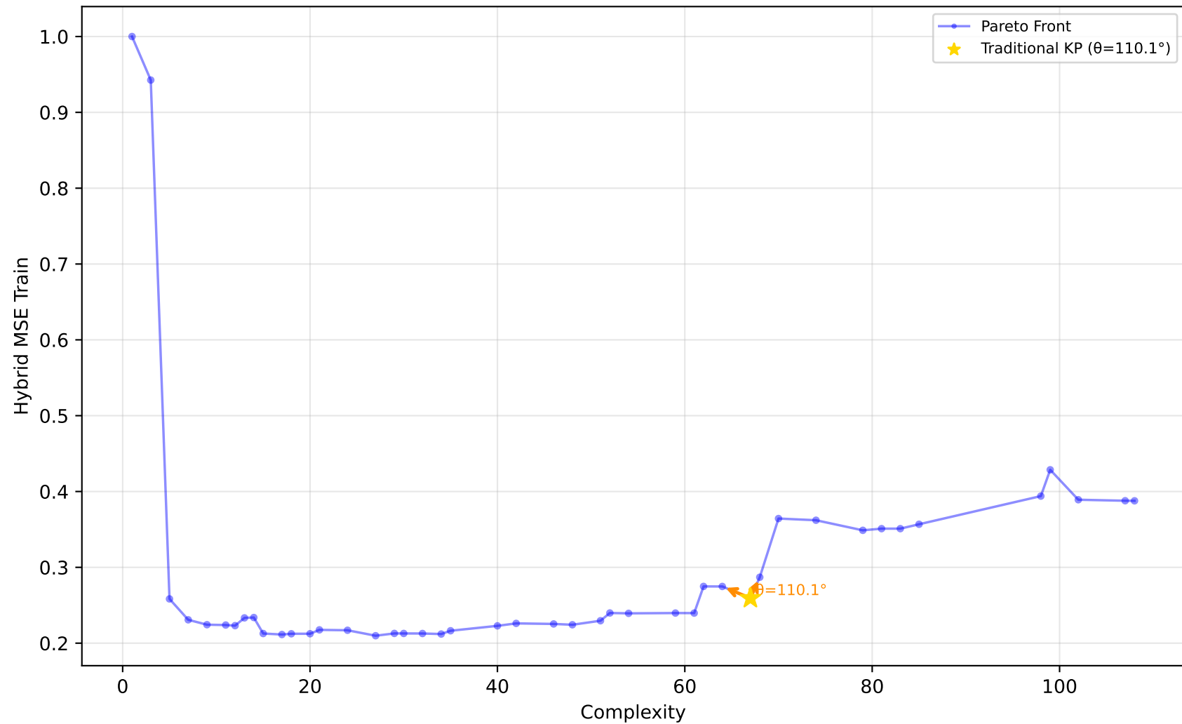
712_chscase_geyser1 - Run 9 - SVP - Hybrid MSE Train \lambda_1=1.00, \lambda_2=1.00, \lambda_3=0.00 | Difficulty: 1.00 | Method: hmr
