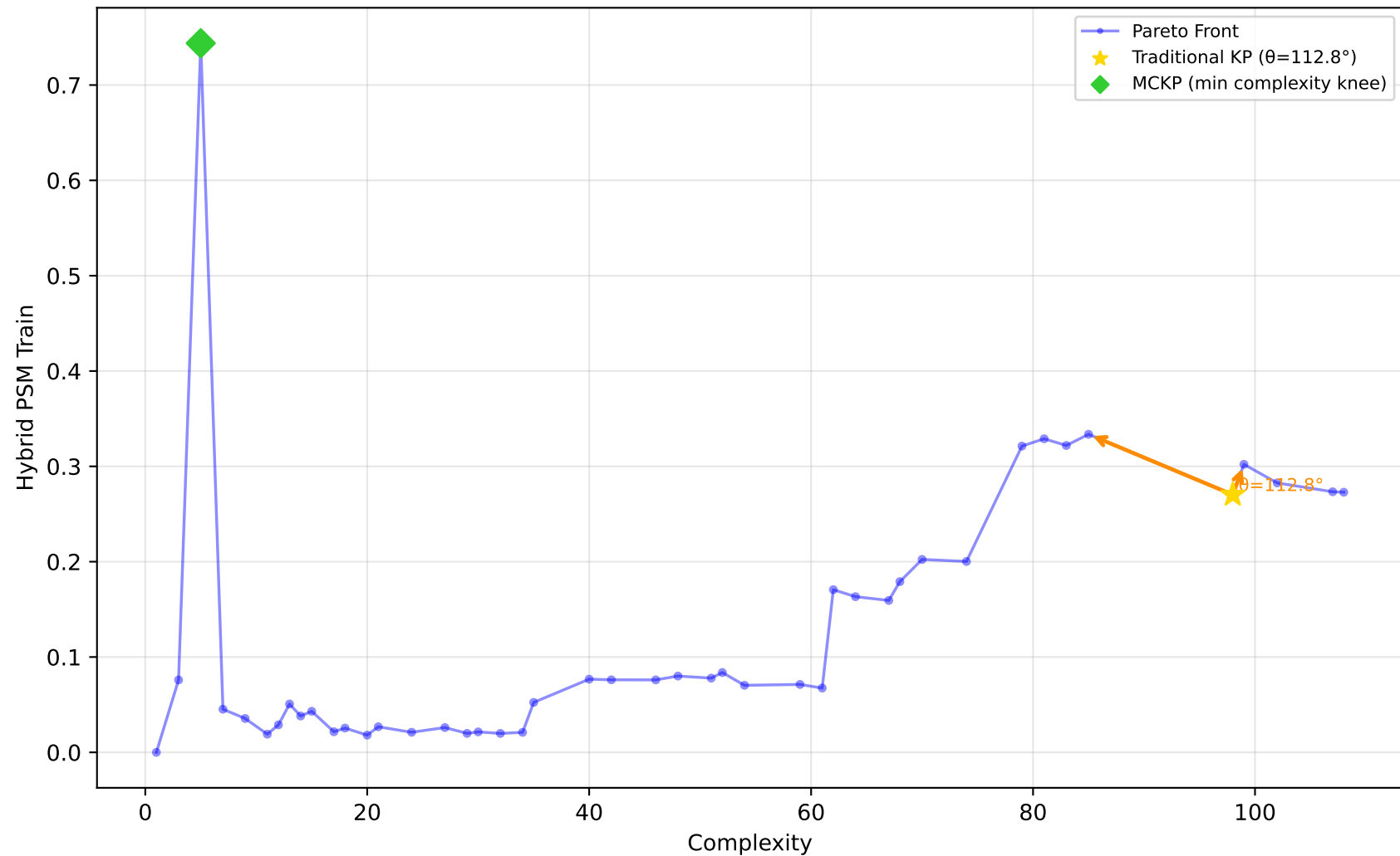
712_chscase_geyser1 - Run 9 - SVP - Hybrid PSM Train \lambda_1=0.00, \lambda_2=1.00, \lambda_3=1.00 | Difficulty: 1.00 | Method: hmr
