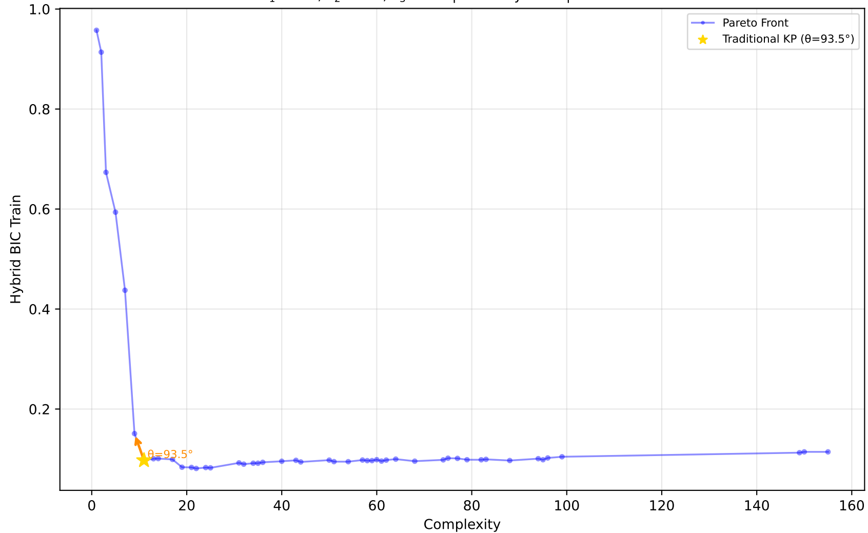
529_pollen - Run 10 - MVP - Hybrid BIC Train \lambda_1=0.00, \lambda_2=1.00, \lambda_3=0.80 | Difficulty: 1.00 | Method: hmr
