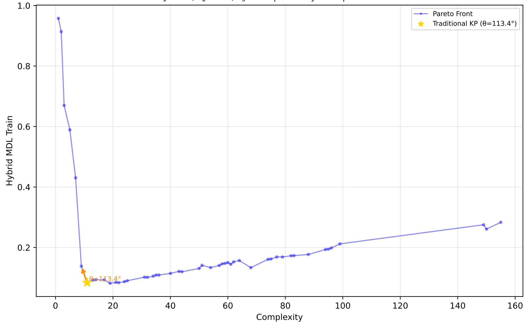
529_pollen - Run 10 - MVP - Hybrid MDL Train \lambda_1=0.00, \lambda_2=1.00, \lambda_3=0.80 | Difficulty: 1.00 | Method: hmr
