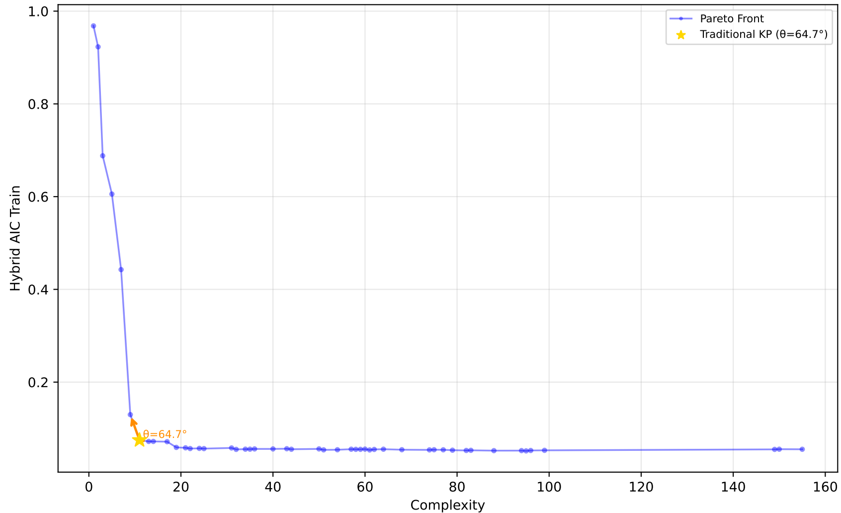
529_pollen - Run 10 - SVP - Hybrid AIC Train \lambda_1=0.10 , \lambda_2=0.80 , \lambda_3=0.30 | Difficulty: 1.00 | Method: hmr
