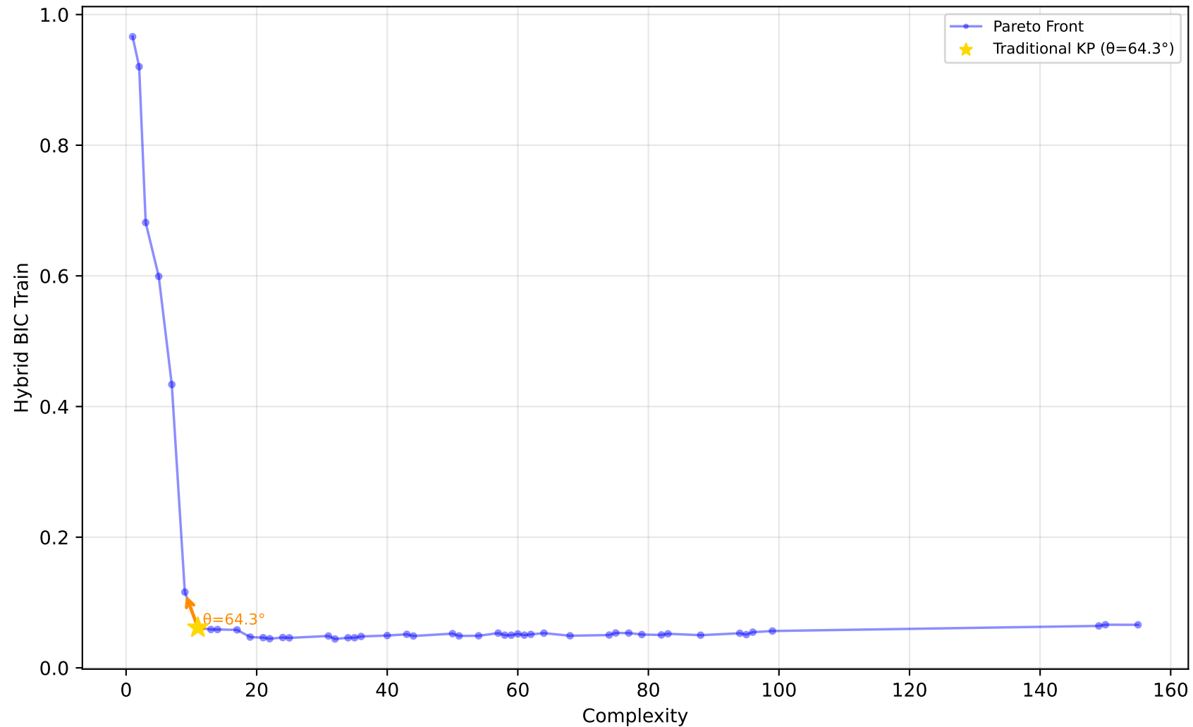
529_pollen - Run 10 - SVP - Hybrid BIC Train \lambda_1=0.10 , \lambda_2=0.80 , \lambda_3=0.30 | Difficulty: 1.00 | Method: hmr
