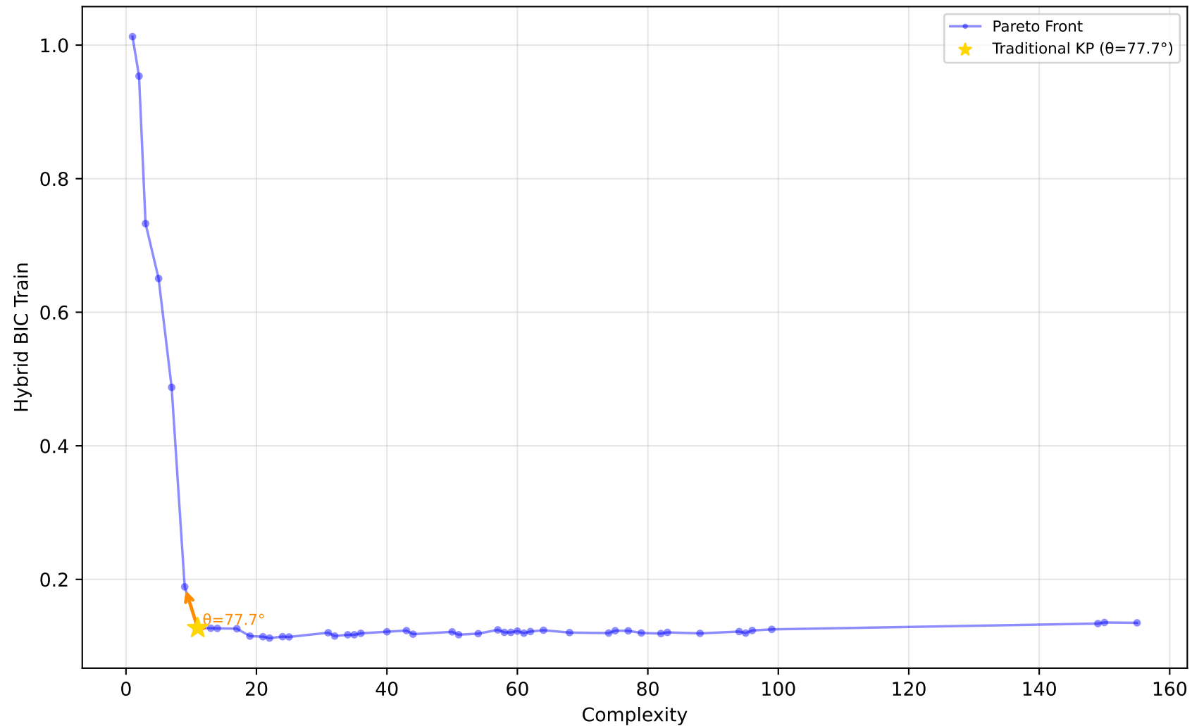
529_pollen - Run 10 - SVP - Hybrid BIC Train \lambda_1=0.60, \lambda_2=0.40, \lambda_3=1.00 | Difficulty: 1.00 | Method: hmr
