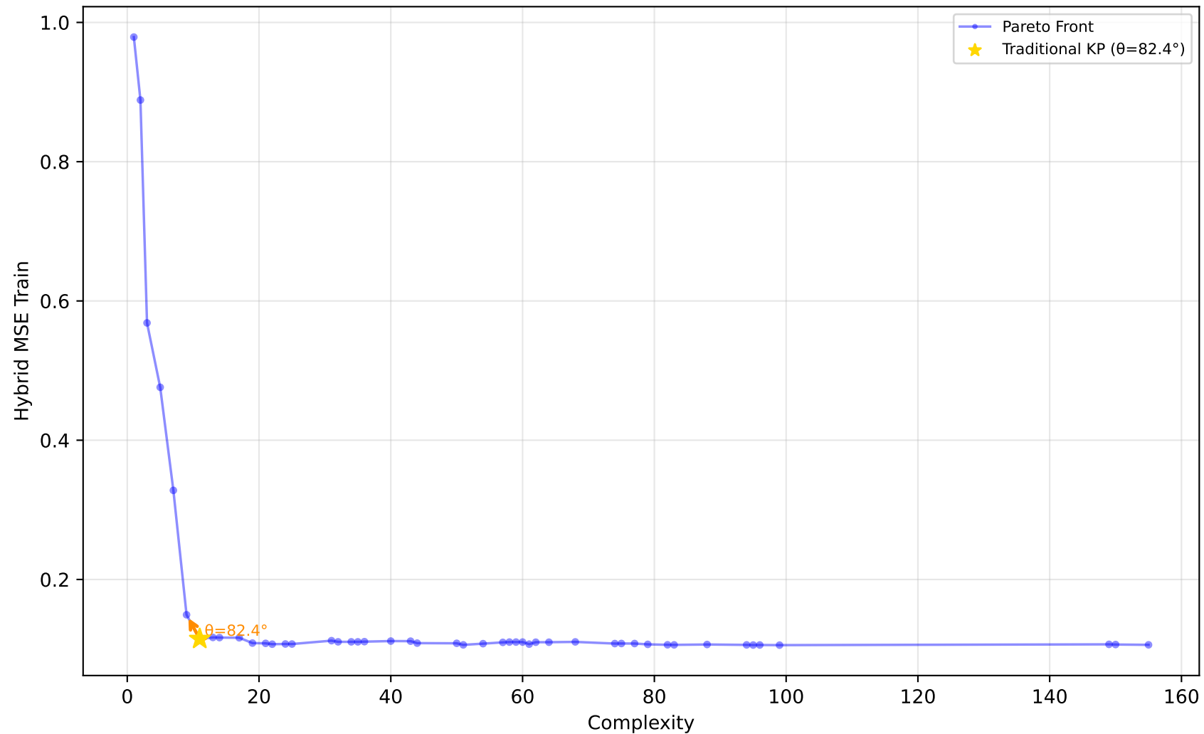
529_pollen - Run 10 - SVP - Hybrid MSE Train \lambda_1=0.60, \lambda_2=0.40, \lambda_3=1.00 | Difficulty: 1.00 | Method: hmr
