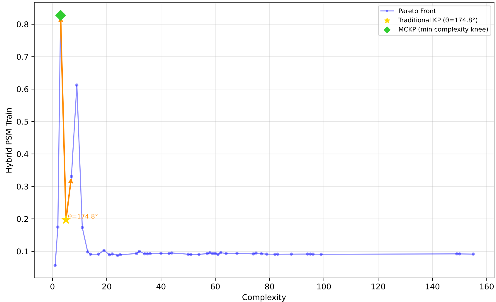
529_pollen - Run 10 - SVP - Hybrid PSM Train \lambda_1=0.60, \lambda_2=0.40, \lambda_3=1.00 | Difficulty: 1.00 | Method: hmr
