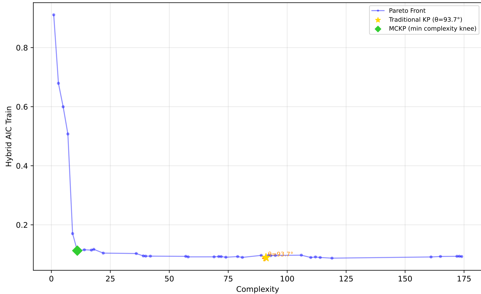
529_pollen - Run 11 - MVP - Hybrid AIC Train \lambda_1=0.00, \lambda_2=1.00, \lambda_3=0.80 | Difficulty: 1.00 | Method: hmr
