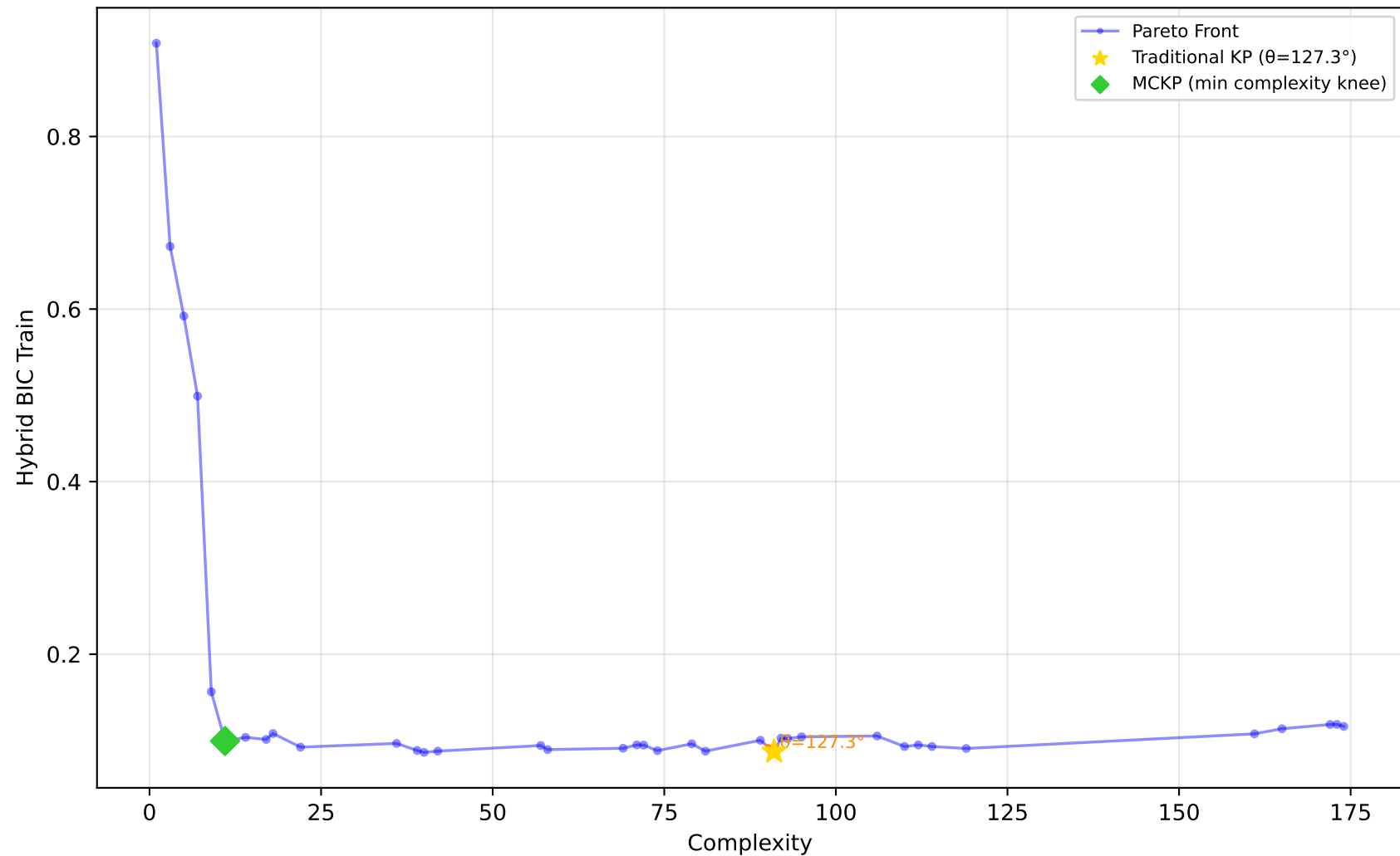
529_pollen - Run 11 - MVP - Hybrid BIC Train \lambda_1=0.00, \lambda_2=1.00, \lambda_3=0.80 | Difficulty: 1.00 | Method: hmr
