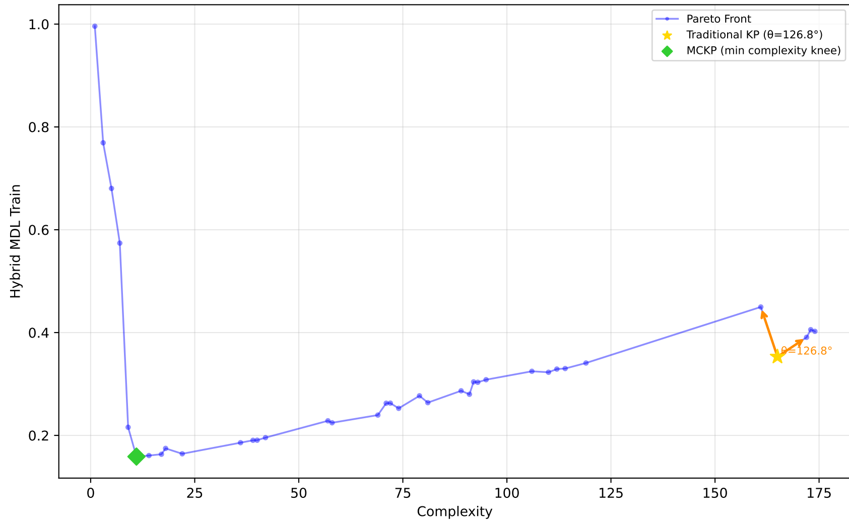
529_pollen - Run 11 - MVP - Hybrid MDL Train \lambda_1=0.90, \lambda_2=0.00, \lambda_3=0.00 | Difficulty: 1.00 | Method: hmr
