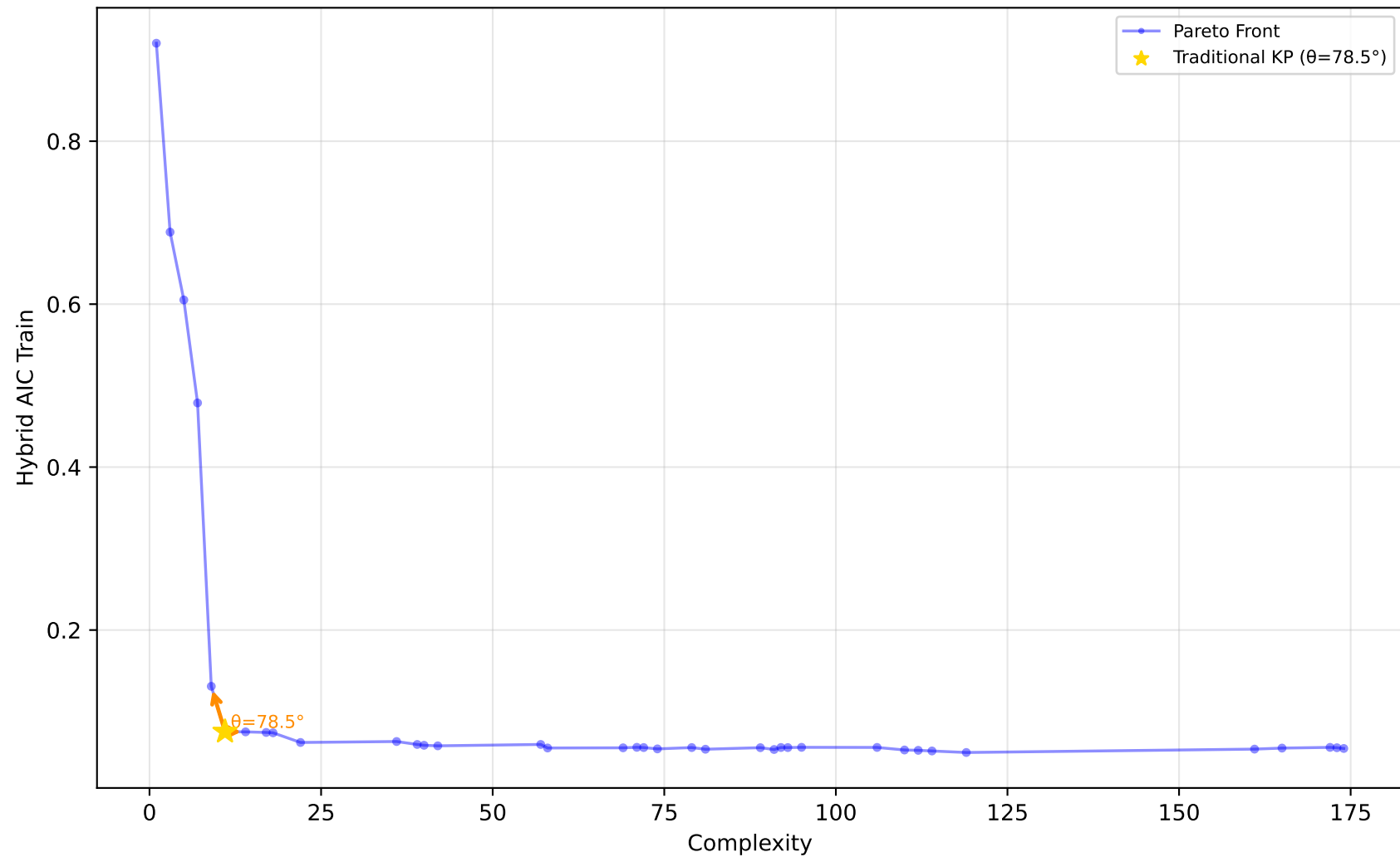
529_pollen - Run 11 - SVP - Hybrid AIC Train \lambda_1=0.10, \lambda_2=0.80, \lambda_3=0.30 | Difficulty: 1.00 | Method: hmr
