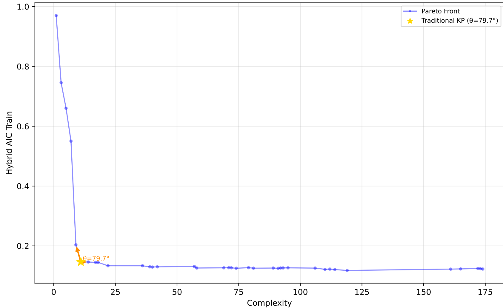
529_pollen - Run 11 - SVP - Hybrid AIC Train \lambda_1=0.60, \lambda_2=0.40, \lambda_3=1.00 | Difficulty: 1.00 | Method: hmr
