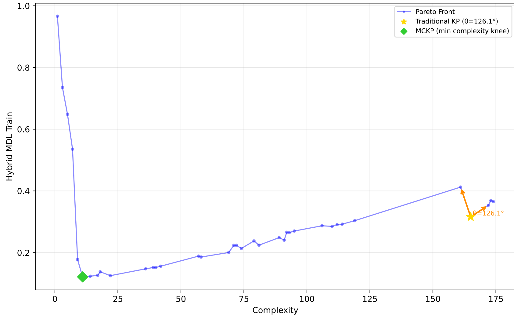
529_pollen - Run 11 - SVP - Hybrid MDL Train \lambda_1=0.60, \lambda_2=0.40, \lambda_3=1.00 | Difficulty: 1.00 | Method: hmr
