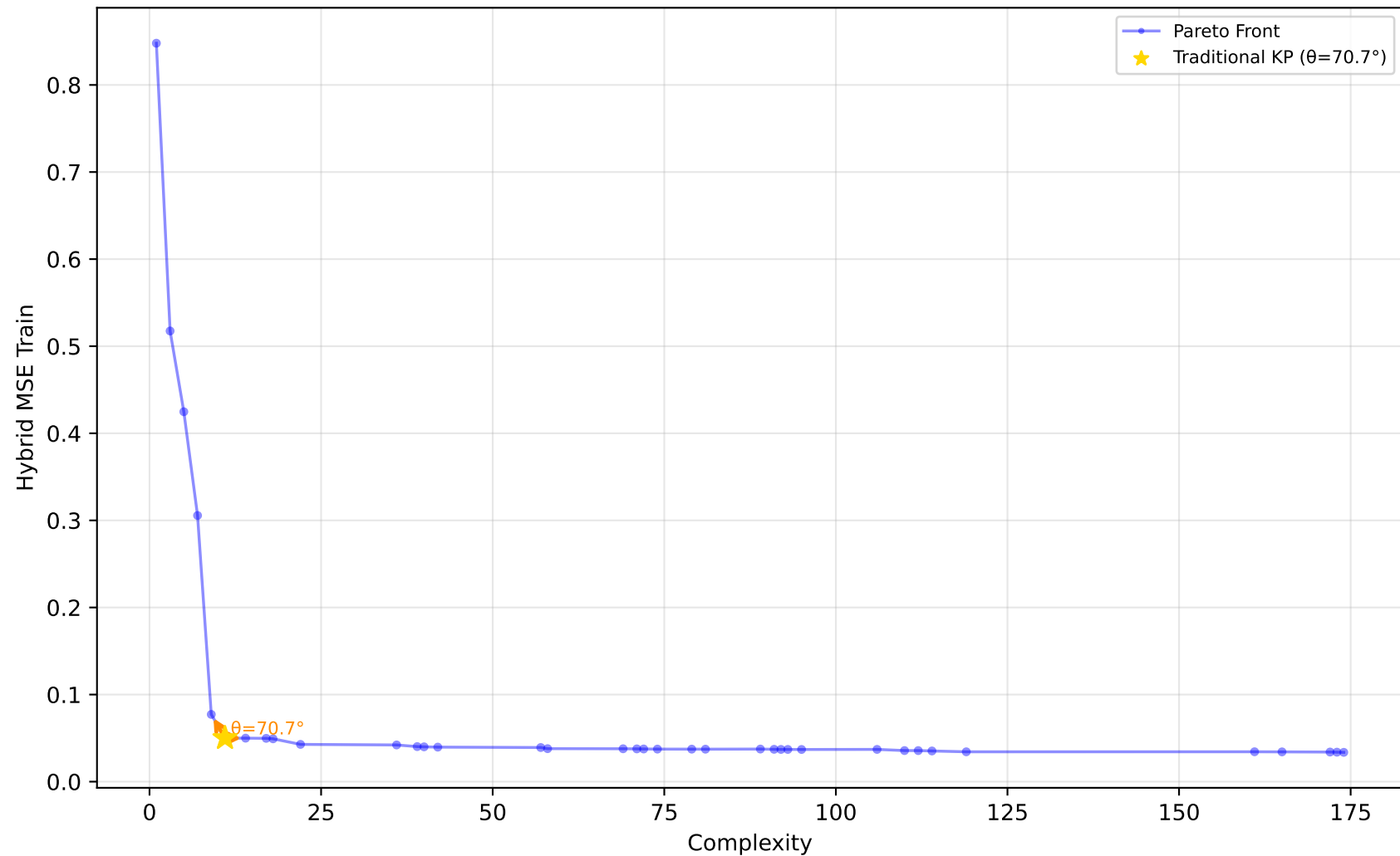
529_pollen - Run 11 - SVP - Hybrid MSE Train \lambda_1=0.10, \lambda_2=0.80, \lambda_3=0.30 | Difficulty: 1.00 | Method: hmr
