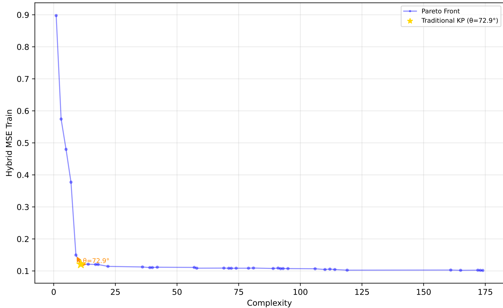
529_pollen - Run 11 - SVP - Hybrid MSE Train \lambda_1=0.60, \lambda_2=0.40, \lambda_3=1.00 | Difficulty: 1.00 | Method: hmr
