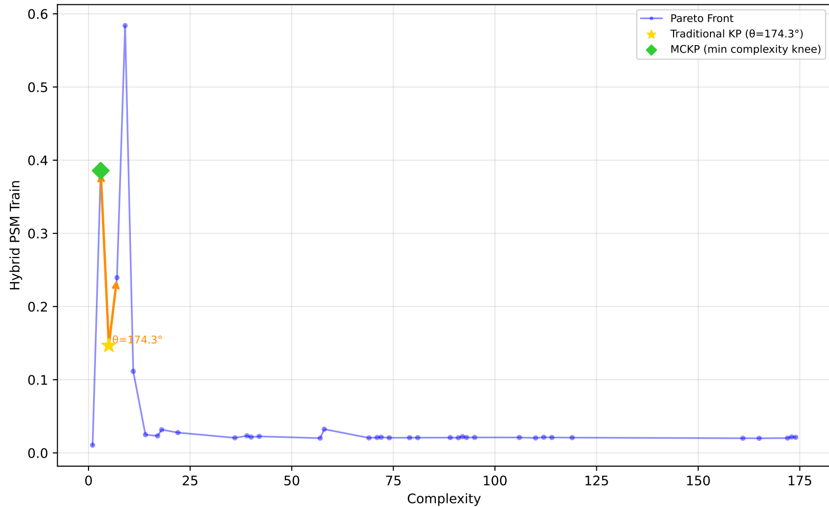
529_pollen - Run 11 - SVP - Hybrid PSM Train \lambda_1=0.10, \lambda_2=0.80, \lambda_3=0.30 | Difficulty: 1.00 | Method: hmr
