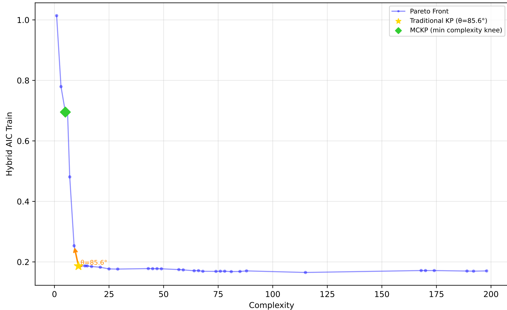
529_pollen - Run 12 - MVP - Hybrid AIC Train \lambda_1=0.90, \lambda_2=0.00, \lambda_3=0.00 | Difficulty: 1.00 | Method: hmr
