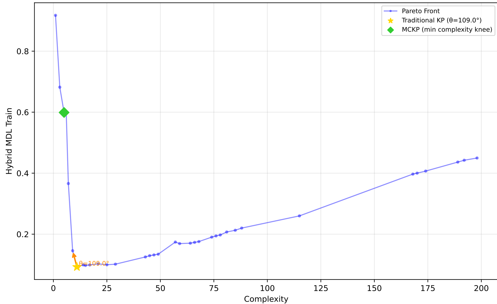
529_pollen - Run 12 - MVP - Hybrid MDL Train \lambda_1=0.00 , \lambda_2=1.00 , \lambda_3=0.80 | Difficulty: 1.00 | Method: hmr
