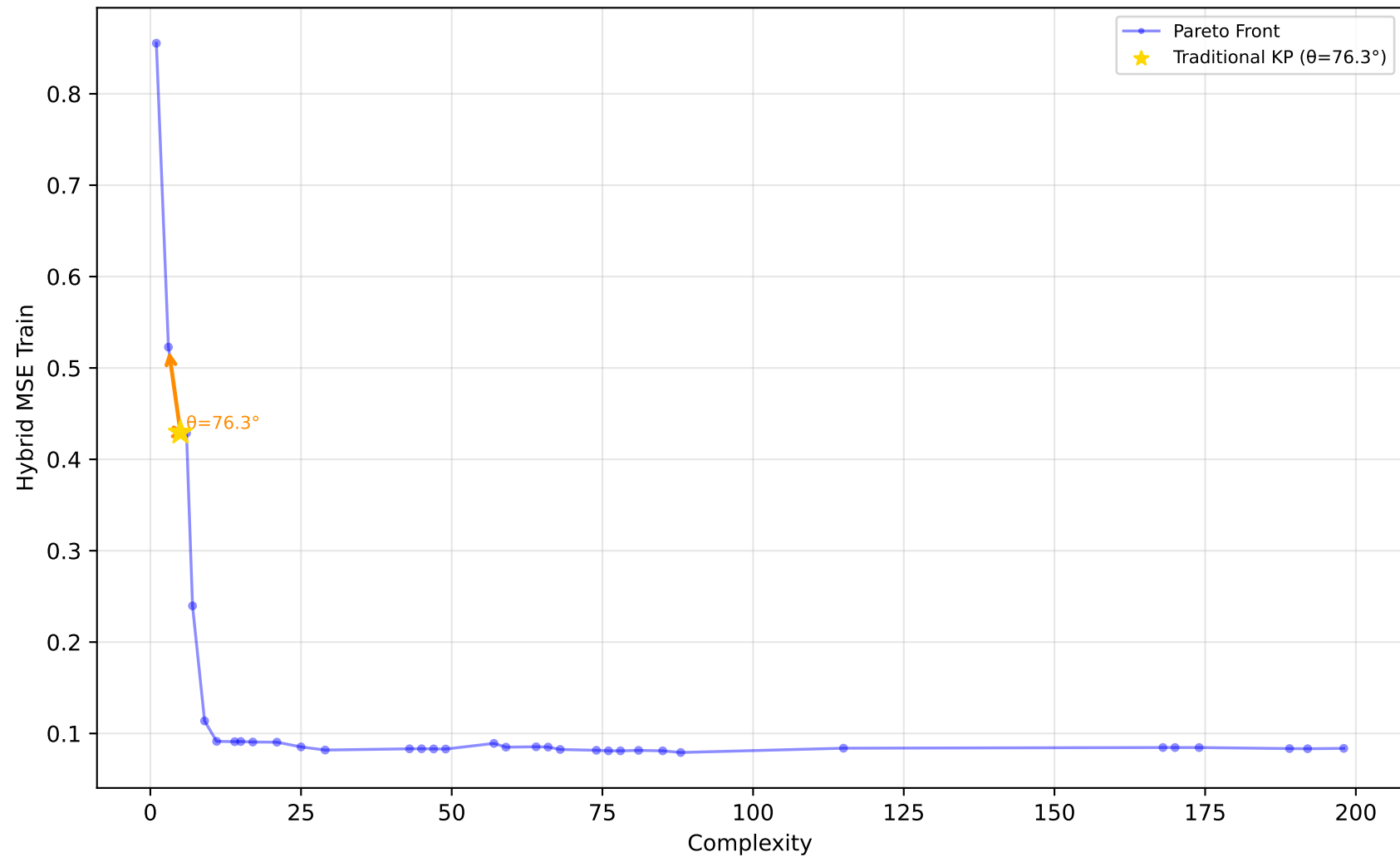
529_pollen - Run 12 - MVP - Hybrid MSE Train \lambda_1=0.00, \lambda_2=1.00, \lambda_3=0.80 | Difficulty: 1.00 | Method: hmr
