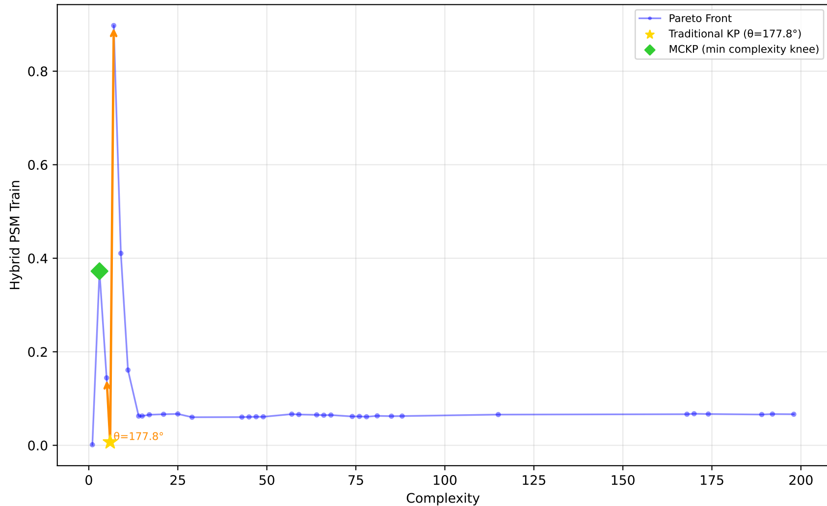
529_pollen - Run 12 - MVP - Hybrid PSM Train \lambda_1=0.00, \lambda_2=1.00, \lambda_3=0.80 | Difficulty: 1.00 | Method: hmr
