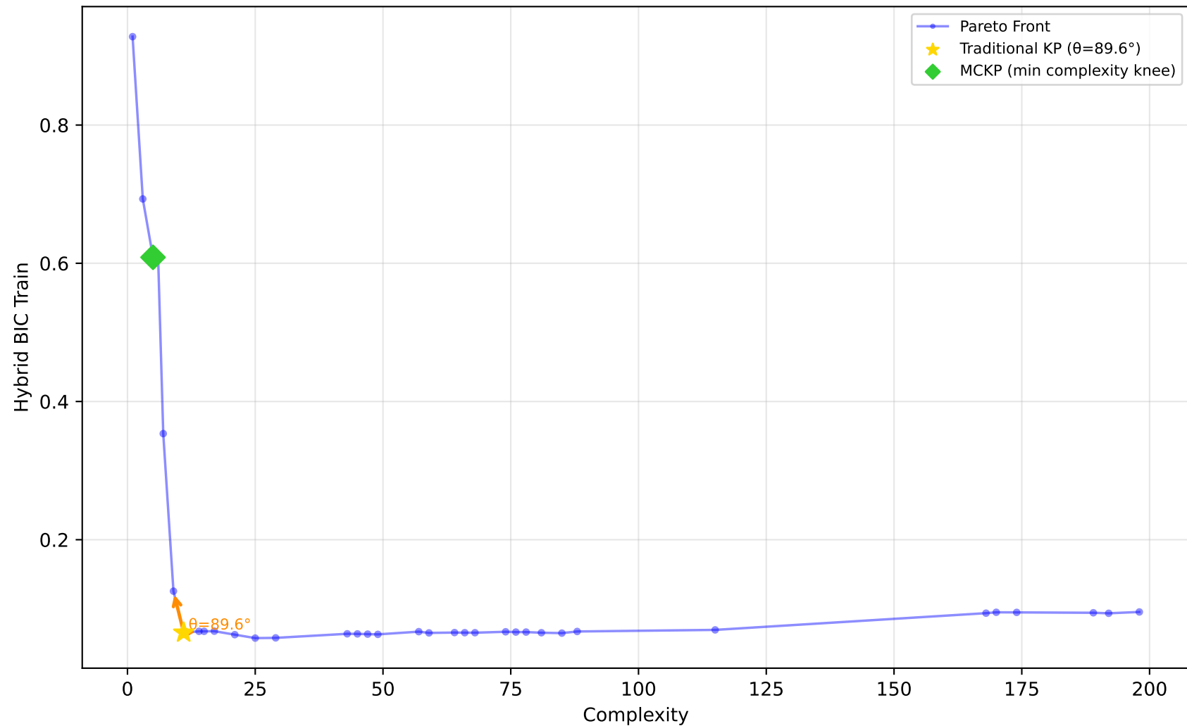
529_pollen - Run 12 - SVP - Hybrid BIC Train \lambda_1=0.10, \lambda_2=0.80, \lambda_3=0.30 | Difficulty: 1.00 | Method: hmr
