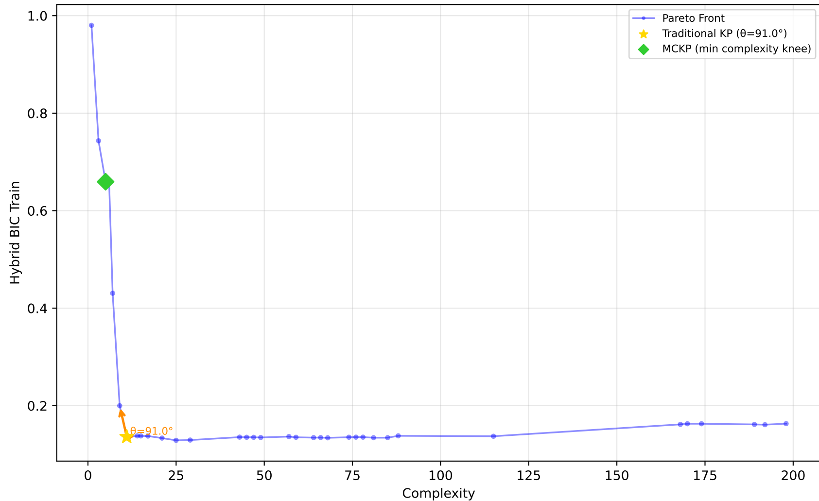
529_pollen - Run 12 - SVP - Hybrid BIC Train \lambda_1=0.60, \lambda_2=0.40, \lambda_3=1.00 | Difficulty: 1.00 | Method: hmr
