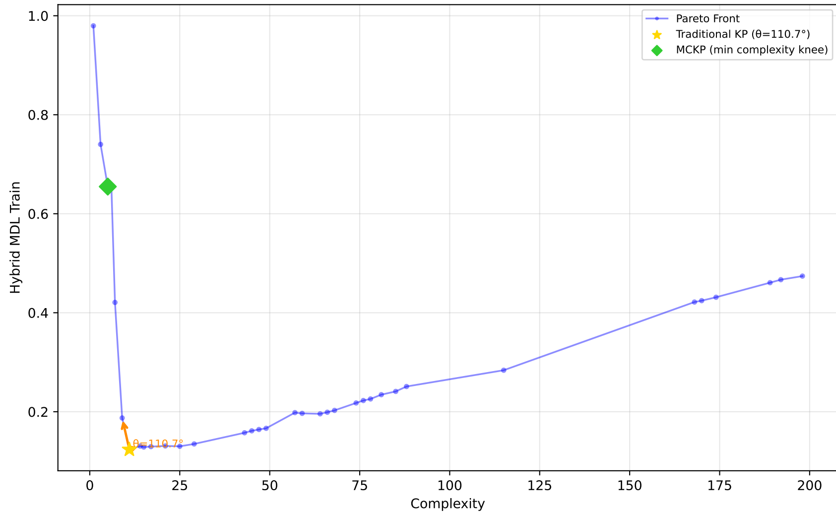
529_pollen - Run 12 - SVP - Hybrid MDL Train \lambda_1=0.60, \lambda_2=0.40, \lambda_3=1.00 | Difficulty: 1.00 | Method: hmr
