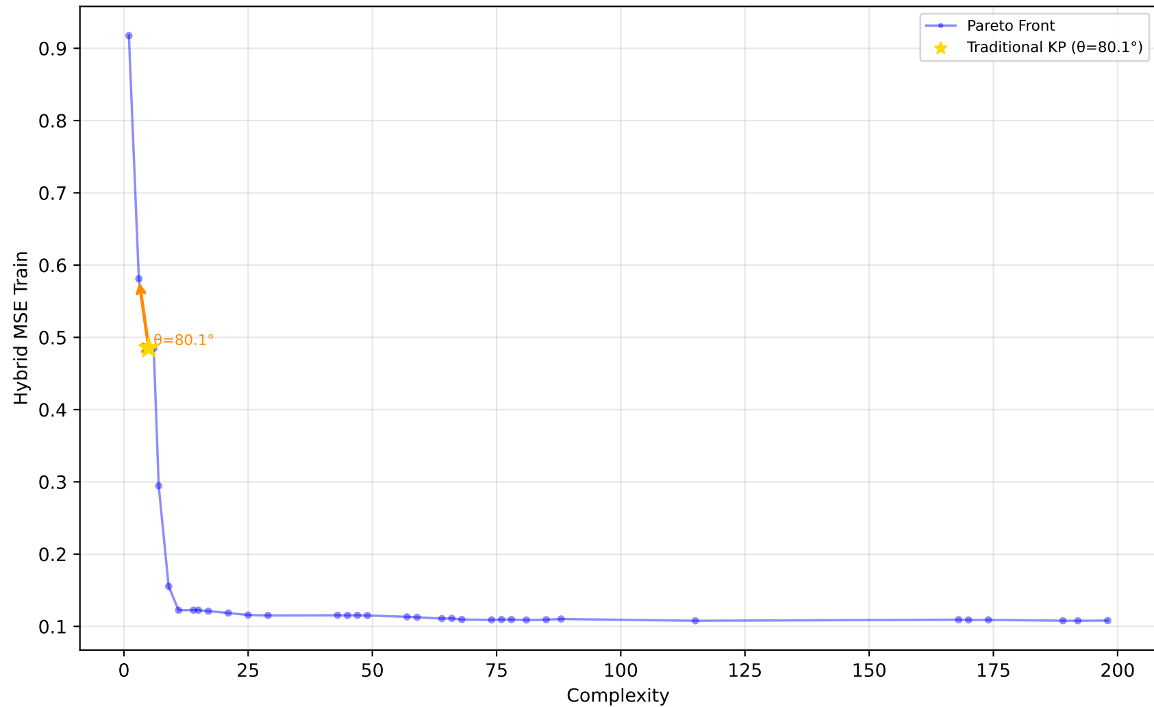
529_pollen - Run 12 - SVP - Hybrid MSE Train \lambda_1=0.60, \lambda_2=0.40, \lambda_3=1.00 | Difficulty: 1.00 | Method: hmr
