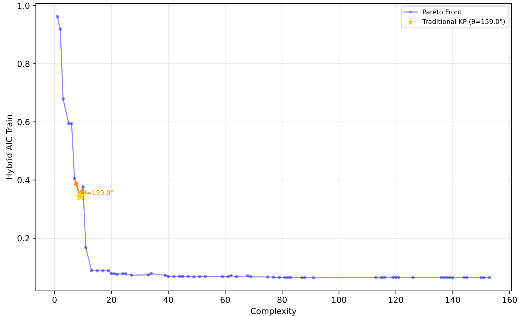
529_pollen - Run 13 - MVP - Hybrid AIC Train \lambda_1=0.00, \lambda_2=1.00, \lambda_3=0.80 | Difficulty: 1.00 | Method: hmr
