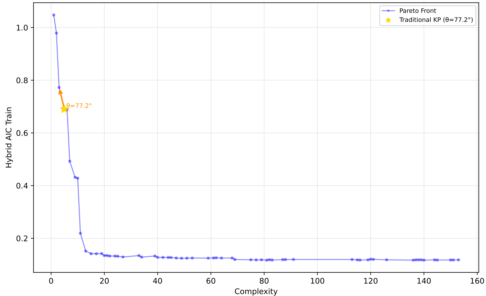
529_pollen - Run 13 - MVP - Hybrid AIC Train \lambda_1=0.90, \lambda_2=0.00, \lambda_3=0.00 | Difficulty: 1.00 | Method: hmr
