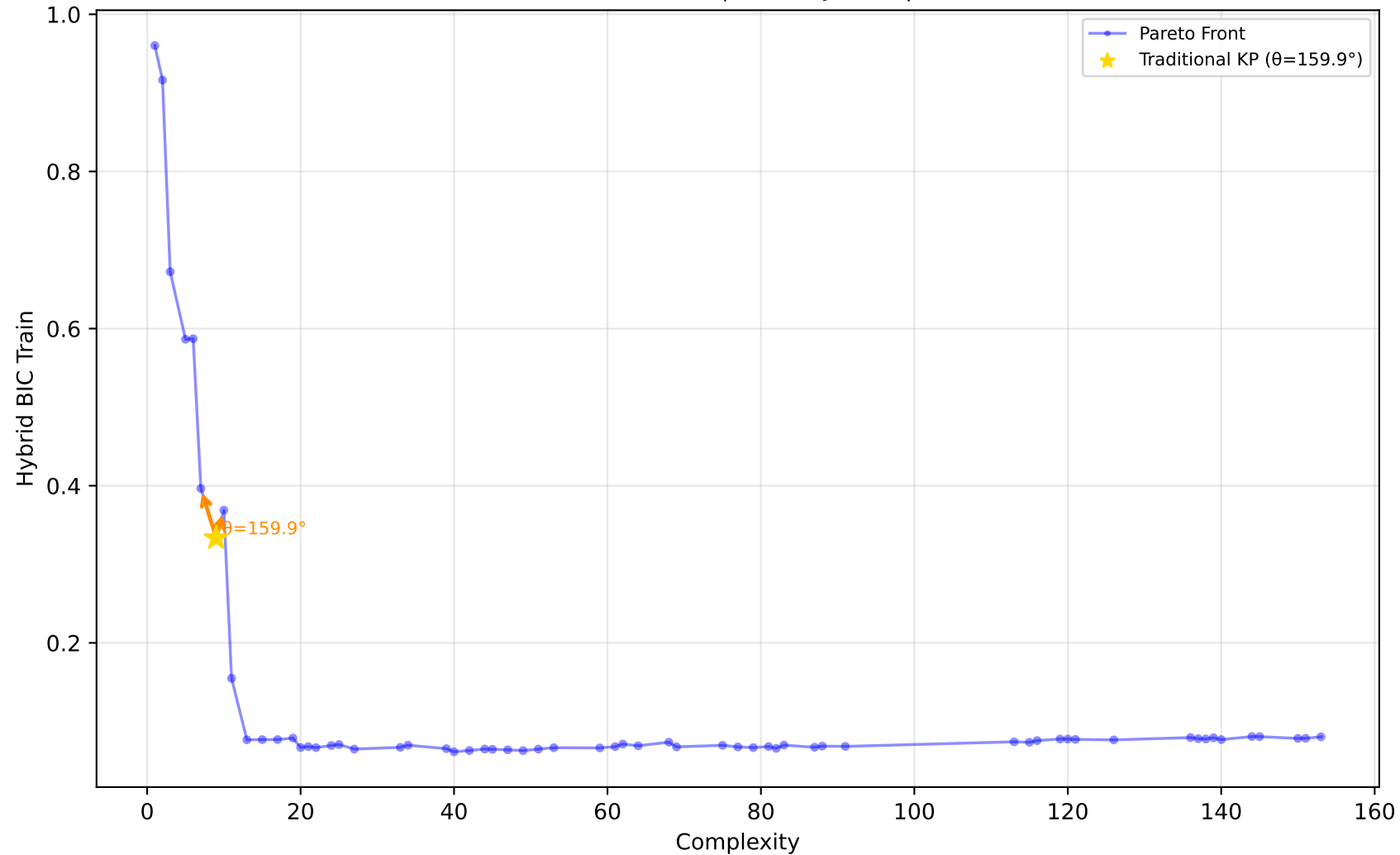
529_pollen - Run 13 - MVP - Hybrid BIC Train \lambda_1=0.00, \lambda_2=1.00, \lambda_3=0.80 | Difficulty: 1.00 | Method: hmr
