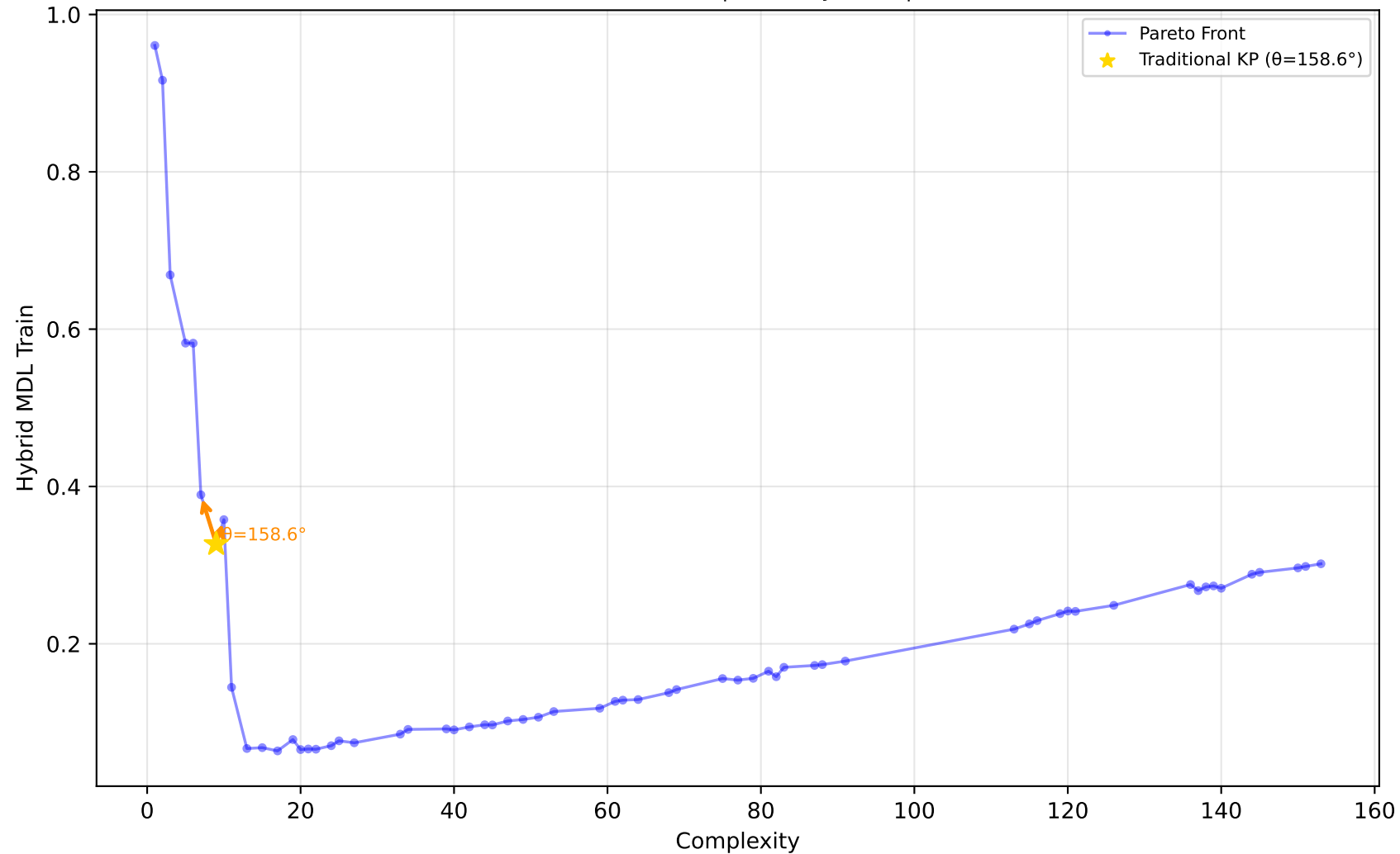
529_pollen - Run 13 - MVP - Hybrid MDL Train \lambda_1=0.00, \lambda_2=1.00, \lambda_3=0.80 | Difficulty: 1.00 | Method: hmr
