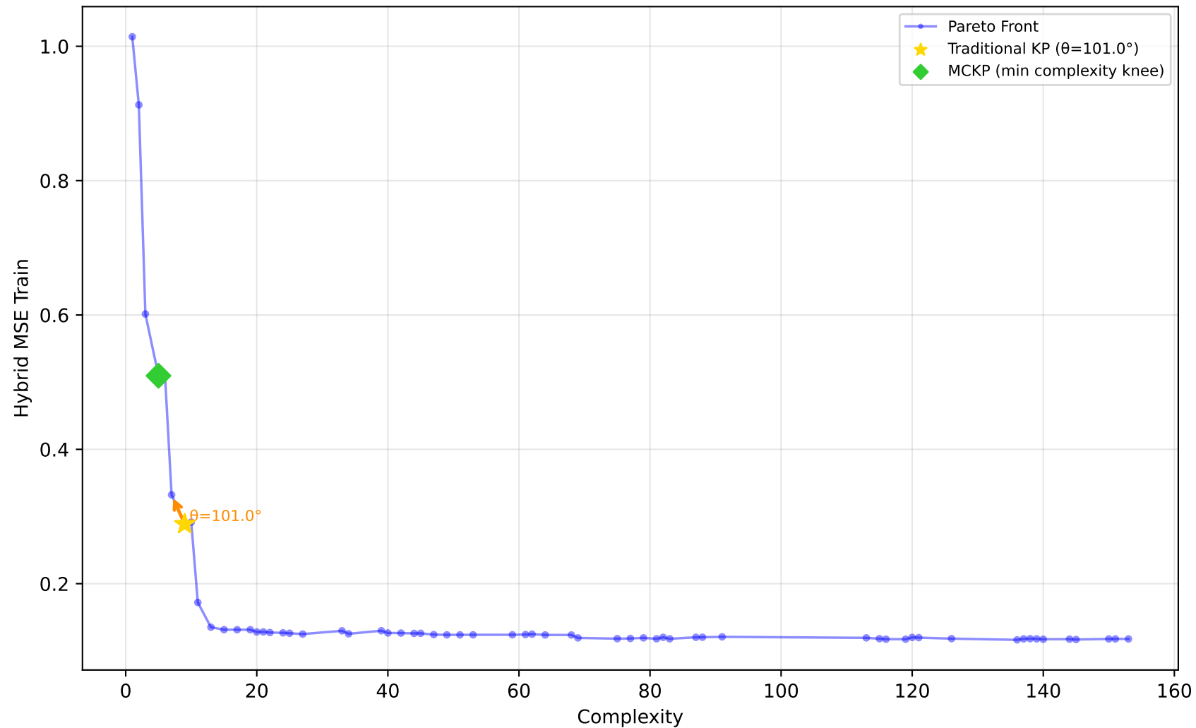
529_pollen - Run 13 - MVP - Hybrid MSE Train \lambda_1=0.90, \lambda_2=0.00, \lambda_3=0.00 | Difficulty: 1.00 | Method: hmr
