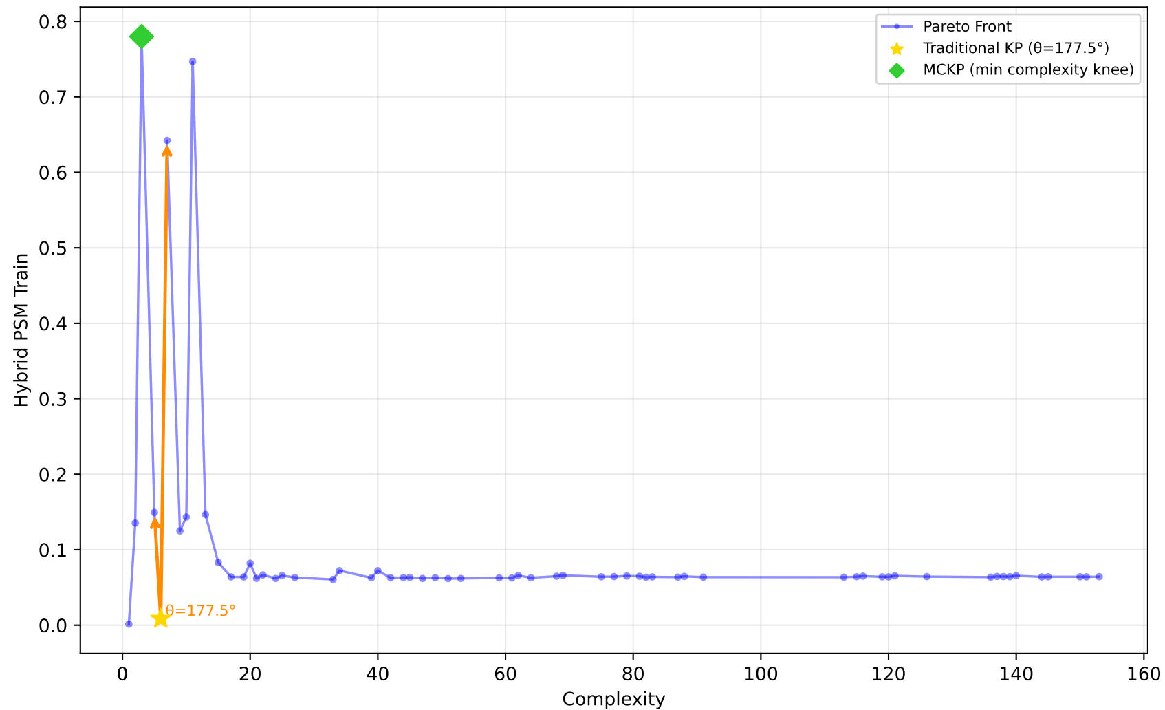
529_pollen - Run 13 - MVP - Hybrid PSM Train \lambda_1=0.00, \lambda_2=1.00, \lambda_3=0.80 | Difficulty: 1.00 | Method: hmr
