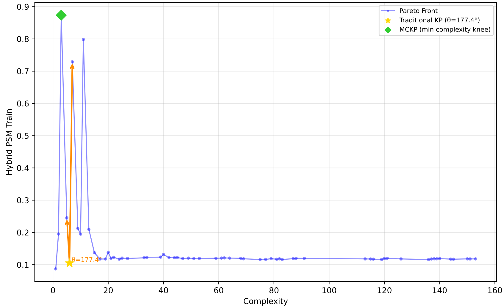
529_pollen - Run 13 - MVP - Hybrid PSM Train \lambda_1=0.90, \lambda_2=0.00, \lambda_3=0.00 | Difficulty: 1.00 | Method: hmr
