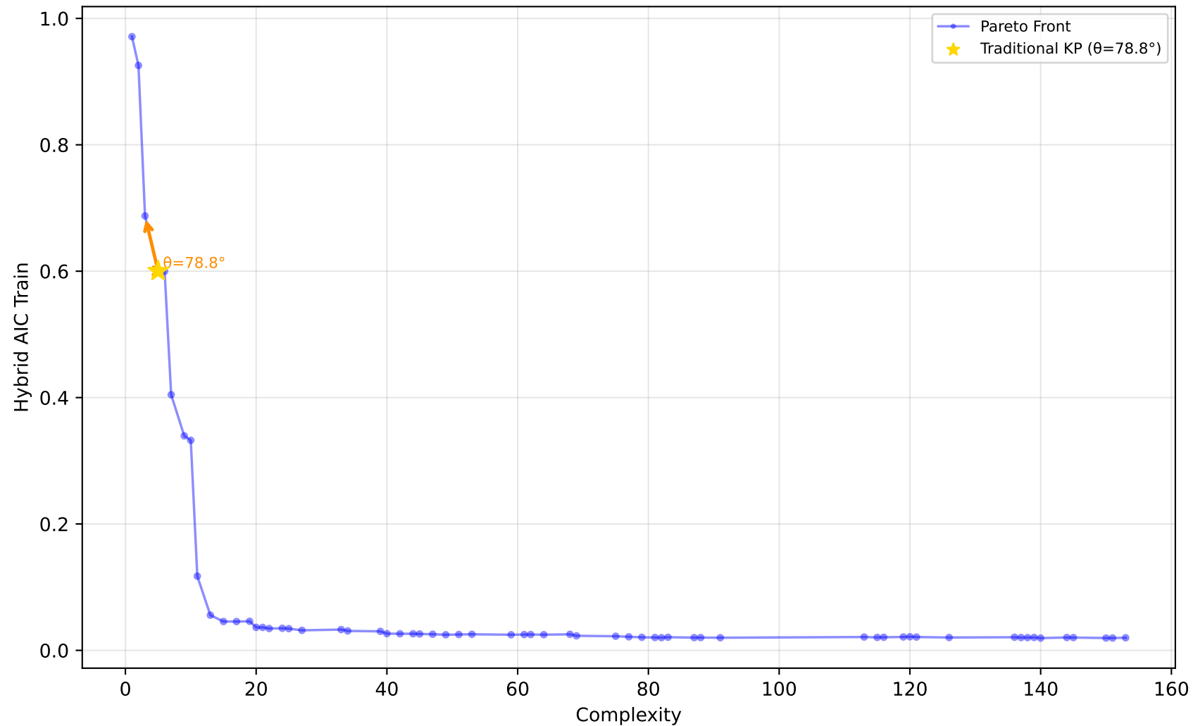
529_pollen - Run 13 - SVP - Hybrid AIC Train \lambda_1=0.10, \lambda_2=0.80, \lambda_3=0.30 | Difficulty: 1.00 | Method: hmr
